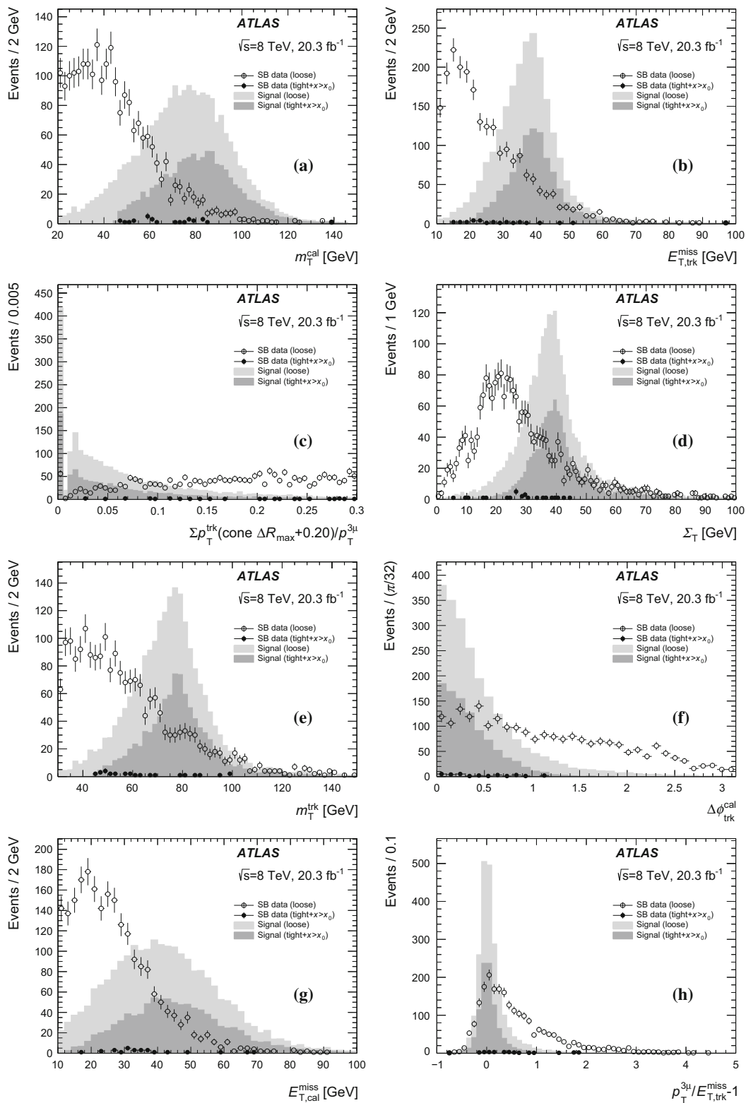
Fig. 2 The BDT inputs ranked 1–8. m_T^{\text{cal}} in a , E_{T,\text{trk}}^{\text{miss}} in b , \Sigma p_T^{\text{trk}}(\Delta R_{\text{max}}^{3\mu} + 0.20) / p_T^{3\mu} in c , \Sigma_T in d , m_T^{\text{trk}} in e , \Delta\phi_{\text{trk}}^{\text{cal}} in f , E_{T,\text{cal}}^{\text{miss}} in g and p_T^{3\mu} / E_{T,\text{trk}}^{\text{miss}} - 1 in h . The loose data in the sidebands are shown as hollow circles, while the loose signal MC events are shown as light solid grey area. The tight+ x > x_0 data in the sidebands are shown as the solid black circles, while the tight+ x > x_0 signal MC events are shown as the
