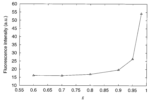
Fig. 3. Effect of anisotropy, g , on the generation of two-photon fluorescence at a focus depth of 200 \mu\text{m} .
