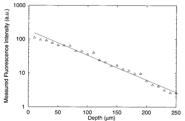
Fig. 6. Measured two-photon fluorescence as a function of focal depth for 0.1- \mu\text{m} fluorescent spheres embedded in a 2% intralipid phantom ( \mu_s^{\text{ex}} = 6 \text{ mm}^{-1} , \mu_s^{\text{em}} = 16 \text{ mm}^{-1} ).
