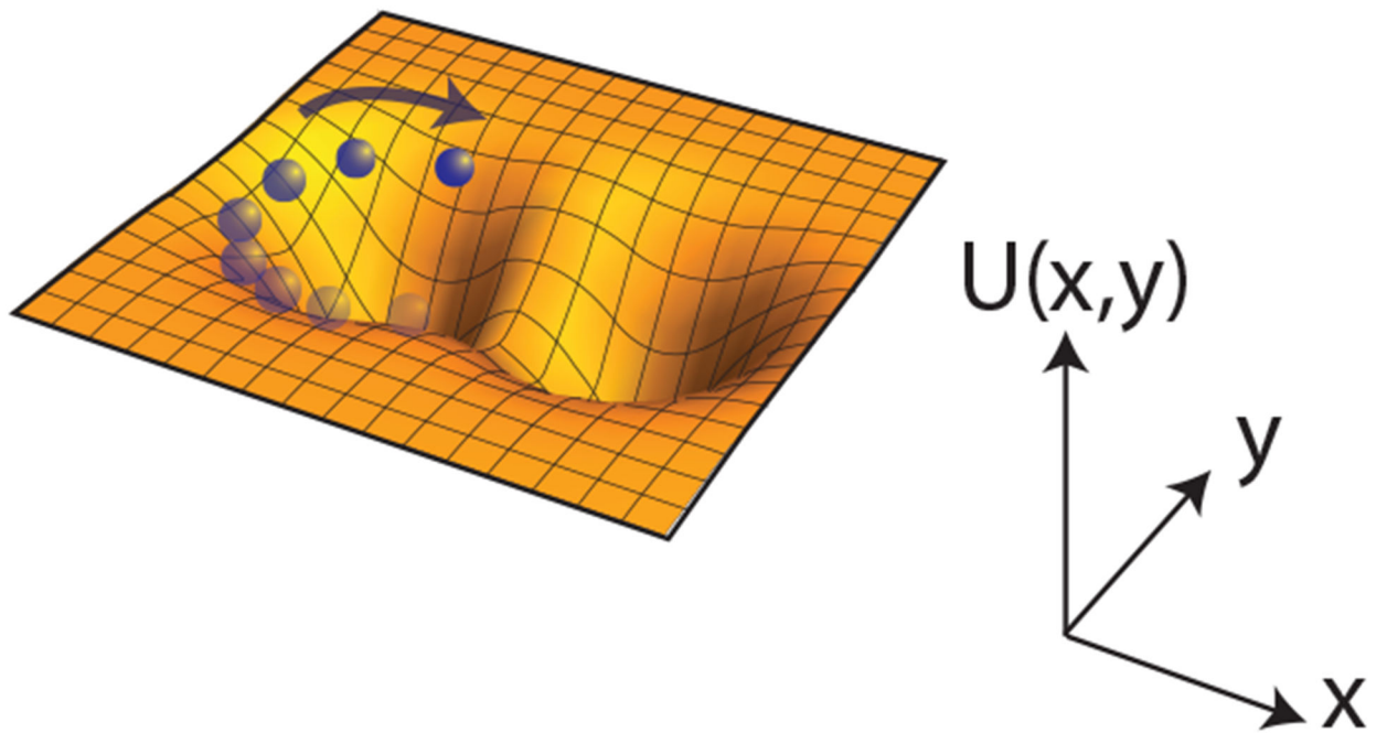
FIG. 5. Schematic representation of a particle moving in a potential landscape with two wells, representing tissue heterogeneities.
