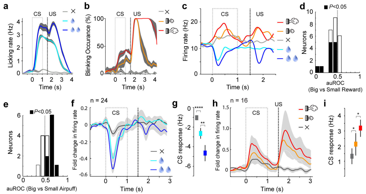
Figure 1. GPh neurons bidirectionally integrate reward and punishment related information a & b, Licking (a) and blinking (b) behaviour from a representative experimental session. The dashed boxed area and dashed line indicate the time of CS and US delivery, respectively. Licking rate ( n = 30 sessions from 7 mice, F(2,18) = 41.59 , P < 0.0001 , P < 0.05 for all comparisons) and blinking occurrence ( n = 32 sessions from 4 mice, F(2,9) = 33.13 , P < 0.001 , P < 0.05 for all comparisons) during the delay between CS and US in recording sessions were compared across different US magnitudes with one-way ANOVA followed by Tukey's test. c, Responses of an example putative GPh neuron, shown as spike density functions. d & e, auROC (area under the Receiver Operating Characteristic) analysis of differences in firing rate between big and small reward trials (d), or between big and small punishment trials (e), during the peak response to the CS presentation (180–480 ms). Filled bars, P < 0.05 , t test. f, Average response of putative GPh neurons to reward. g, Firing rate change during CS predicting reward of different amplitudes (Big vs. Small reward, z = -3.2 , **P < 0.01 ; Small vs. No reward, z = -4.11 , ****P < 0.0001 ; Wilcoxon signed-rank test). h, Average response of putative GPh neurons to punishment. i, Firing rate change during CS predicting punishment of different durations (Big vs. Small punishment, z = 2.27 , *P < 0.05 ; Small vs. No punishment, z = 2.06 , *P < 0.05 , Wilcoxon signed-rank test). Data are represented as mean \pm s.e.m. in a, b, f–i.
