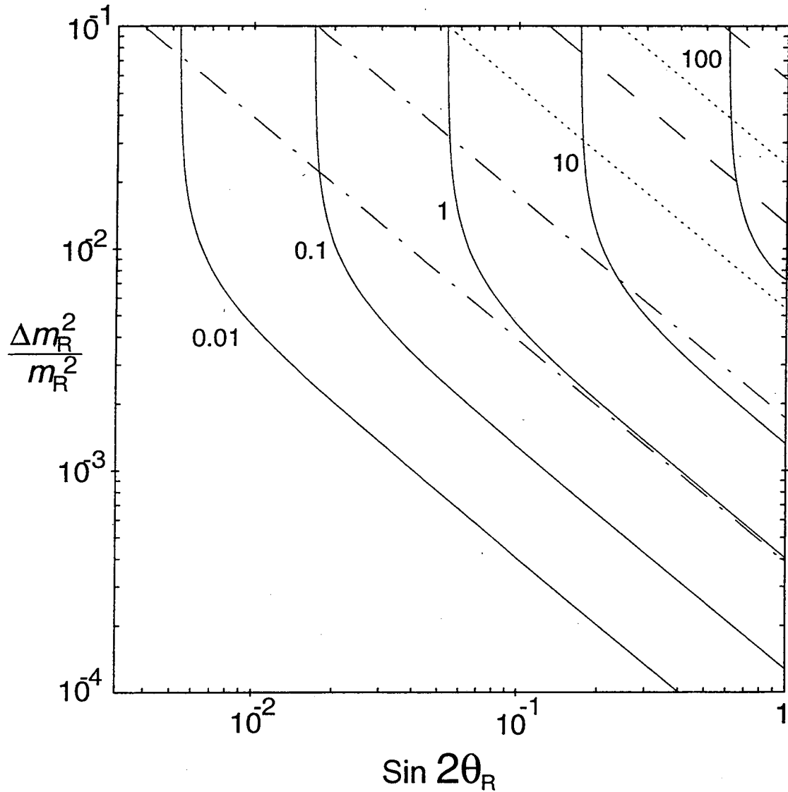
FIG. 2. Contours of constant \sigma(e^+e_R^- \rightarrow e^\pm \mu^\mp \tilde{\chi}^0 \tilde{\chi}^0) (solid) for NLC, with \sqrt{s} = 500 GeV, m_{\tilde{e}_R}, m_{\tilde{\mu}_R} \approx 200 GeV, and M_1 = 100 GeV (solid). Constant contours of B(\mu \rightarrow e\gamma) are also plotted as in Fig. 1, but for left-handed sleptons degenerate at 350 GeV.
