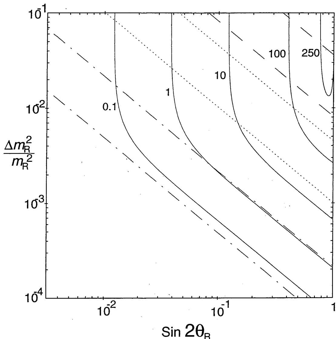
FIG. 1. Contours of constant \sigma(e^+e^- \rightarrow e^\pm \mu^\mp \tilde{\chi}^0 \tilde{\chi}^0) (solid) for LEP II, with \sqrt{s} = 190 GeV, m_{\tilde{e}_R}, m_{\tilde{\mu}_R} \approx 80 GeV, and M_1 = 50 GeV. Constant contours of B(\mu \rightarrow e\gamma) = 4.9 \times 10^{-11} and 2.5 \times 10^{-12} are also plotted for degenerate left-handed sleptons with mass 120 GeV and \tilde{t} \equiv (A + \mu \tan \beta)/\bar{m}_R = 0 (dotted), 2 (dashed), and 50 (dot-dashed).
