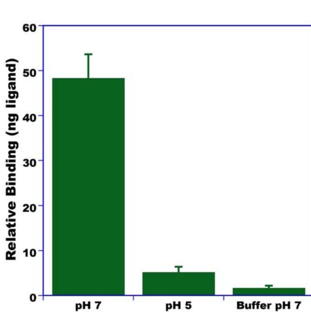
Figure 11. Binding of the major sex pheromone constituent to AtrPB1. Z11Z13-16Ald showed high affinity for the pheromone-binding protein at pH 7, but low or no binding activity at low pH. Minimal non-specific binding is indicated by the low amounts of ligand detected after incubation with buffer only. doi:10.1371/journal.pone.0007235.g011
