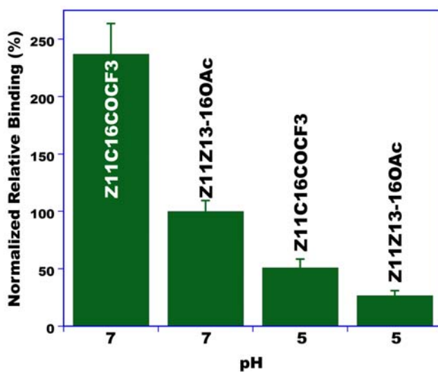
Figure 13. Binding of a pheromone analog to AtrPBPP1. Competitive binding of a pheromone analog, Z11C16COCF 3 , and the best natural ligand, Z11Z13-16OAc. Both ligands at equimolar concentration were incubated with AtrPBPP1 at the same time. AtrPBPP1 bound with much higher affinity to the pheromone analog and even retained the ligand at low pH. doi:10.1371/journal.pone.0007235.g013
