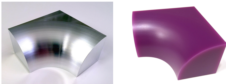
Figure 11: The finished oriented-translation swept surface, using 240 passes with a 0.00005 inch scallop height, in aluminum 6061 (left) and wax (right).
