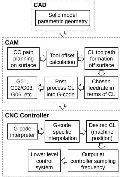
Figure 1: Traditional workflow for CAM-based CNC machining.
