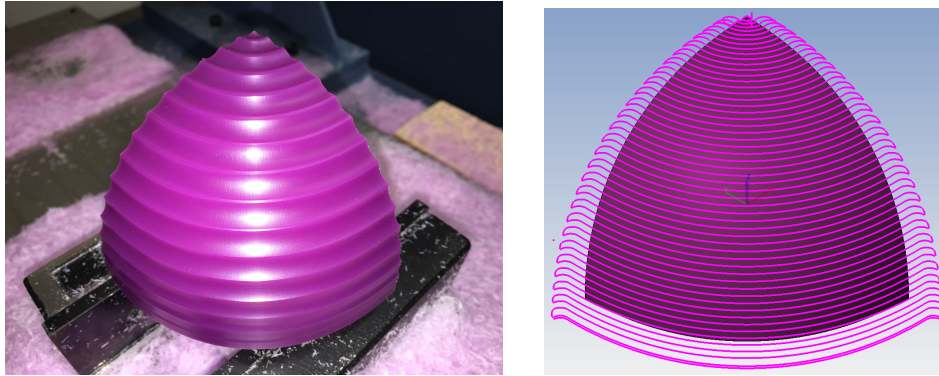
Figure 9: Left: result of a semi-finishing pass with a fixed scallop height for the scaled-rotation swept surface, machined in wax. Right: CAM-generated (G01) surface finishing tool paths — for clarity, the scallop height is greatly increased above the nominal 0.00005 inch value.
