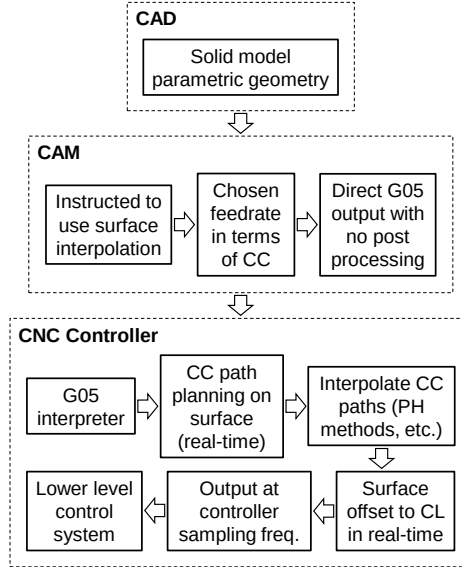
Figure 6: Proposed workflow for the real-time surface interpolator.
