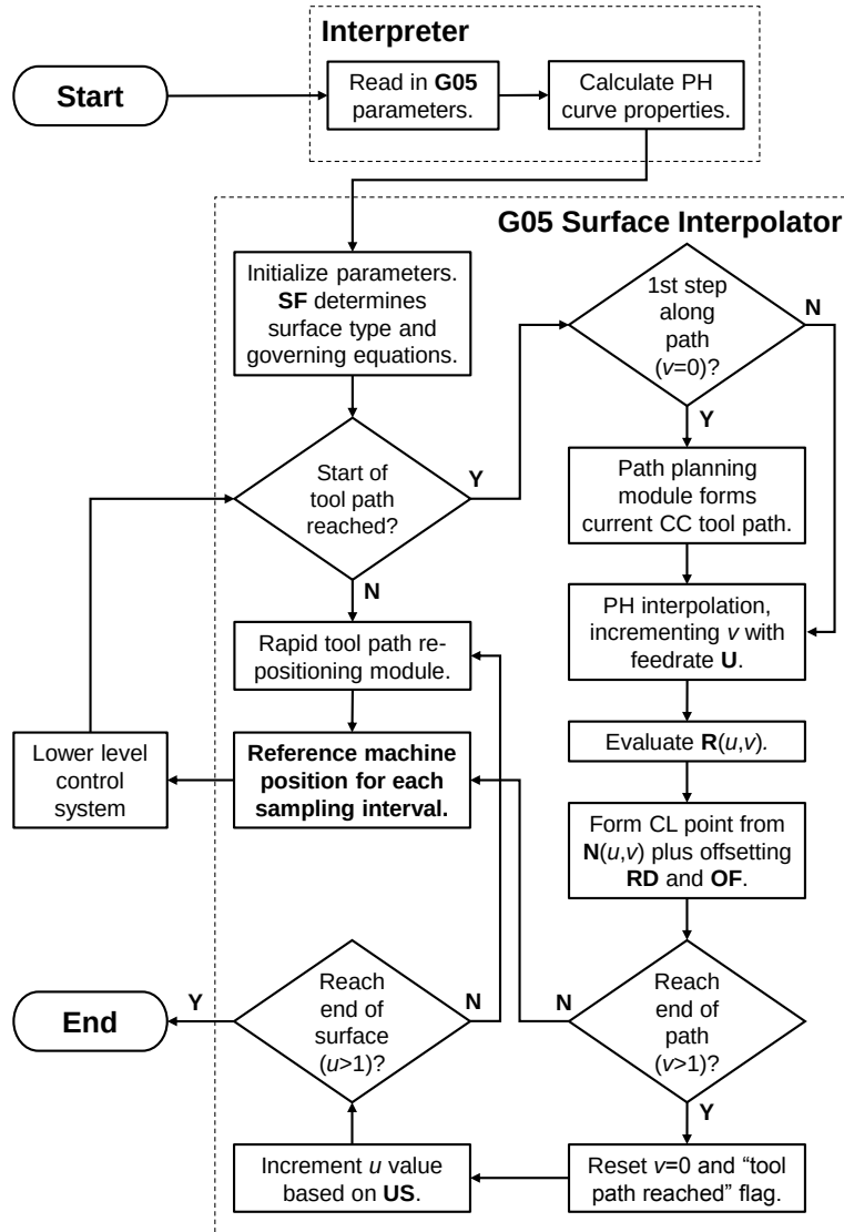
Figure 7: Simplified logic flowchart for the real-time G05 surface interpolator using an iso-parametric tool path machining strategy.
