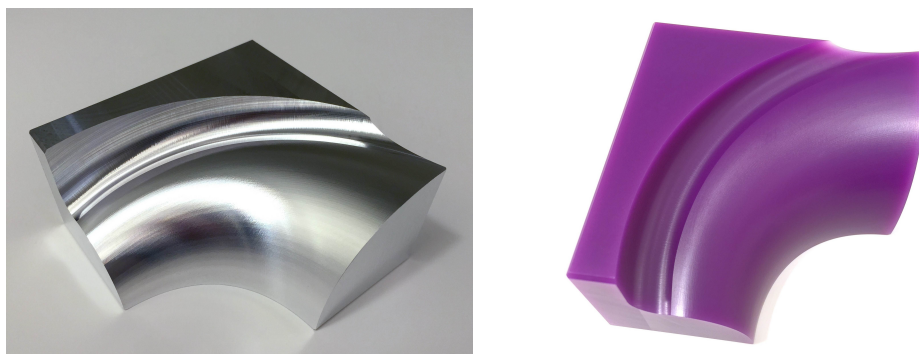
Figure 13: The finished generalized conical swept surface, using 240 passes with a 0.00005 inch scallop height, in aluminum 6061 (left) and wax (right).
