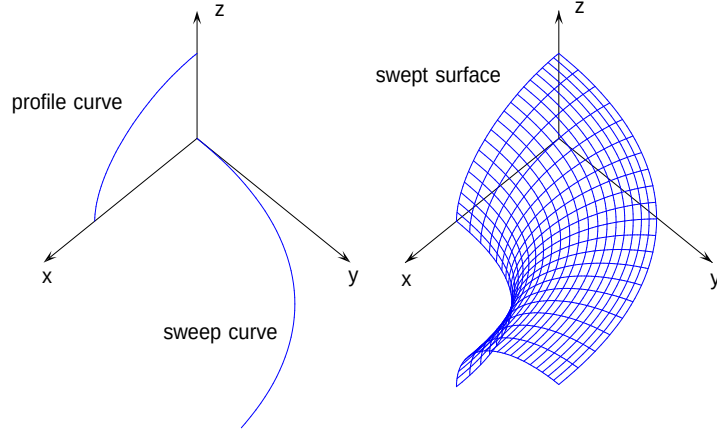
Figure 3: An example of the oriented-translation swept surface.
