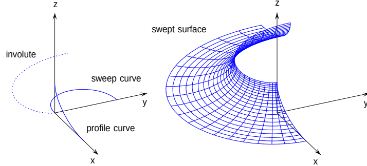
Figure 4: An example of the oriented-involute swept surface.
