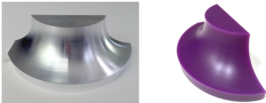
Figure 12: The finished oriented-involute swept surface, using 240 passes with a 0.00005 inch scallop height, in aluminum 6061 (left) and wax (right).
