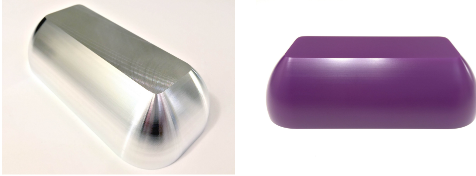
Figure 14: A composite of eight oriented-translation swept surfaces combined into a single G05 command in the SF08 multiple-surface mode (174 passes with a 0.00005 inch scallop height) in aluminum 6061 (left) and wax (right).
