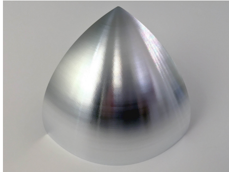
Figure 10: The finished scaled-rotation swept surface with a very fine scallop height of 0.00005 inch, as machined in aluminum 6061 (left) and wax (right).
