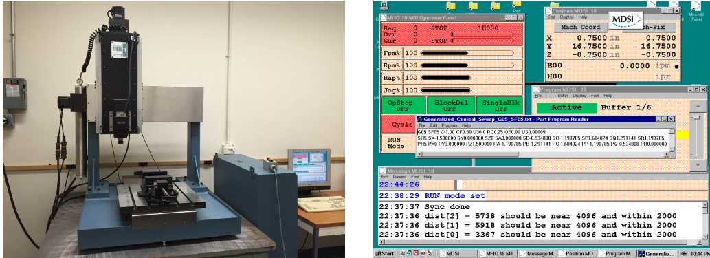
Figure 8: Left: the 3-axis milling machine run by the OpenCNC controller. Right: the controller display of a G05 swept surface program, ready to run the machine through the custom interpolator routine integrated into OpenCNC.
