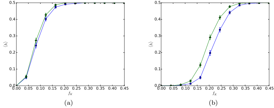
Figure 6: (a) The average normalized Hamming distance is plotted versus fractional mutation frequency, f_K , of equilibrium constants K_{ij} . Diamonds correspond to \beta\delta/N = 4.0 , and squares \beta\delta/N = 8.0 . Here a = b = 0.4 , and \epsilon = \delta = 0.6 (see Eqs. 8 and 10). (b) The same situation with a = b = 0.001 , and \epsilon = \delta = 0.999 .
