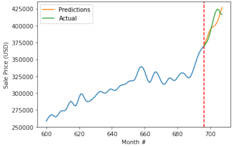
Figure 4.3: LSTM Model Forecast Actual vs. Predicted
