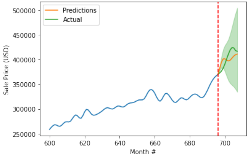
Figure 4.4: ARIMA Model Forecast with 95% Forecast Interval
