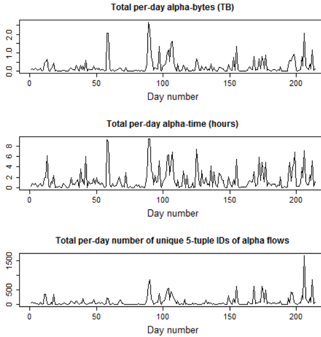
Fig. 5: Cumulative (across all \alpha prefix IDs) per-day data
