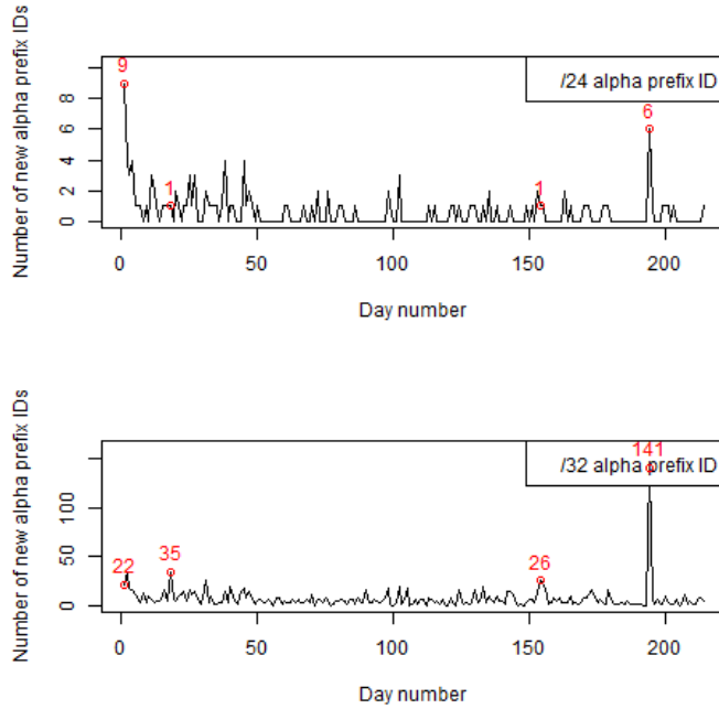
Fig. 8: Number of new \alpha prefix IDs per day
