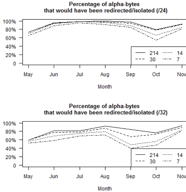
Fig. 10: Effectiveness of AFTES for different values of the aging parameter
