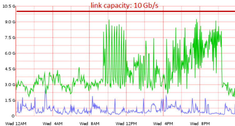
Fig. 1: Utilization (b/s) of a 10 Gbps ESnet router interface observed on Jan. 16, 2013; the green line, showing bursts reaching over 9 Gbps, is the outgoing traffic from the ESnet router to a peering REN, while the lower-load blue line is the incoming traffic on the same interface [6]
