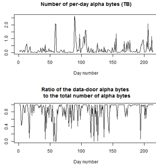
Fig. 15: A measure of the ratio of \alpha -bytes from/to data doors
