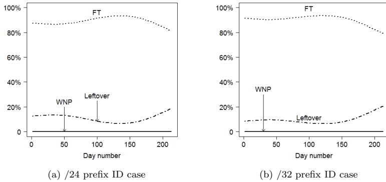
Fig. 13: Percentages of four groups of hapless \beta flow packets with smoothing spline function (df=4)
