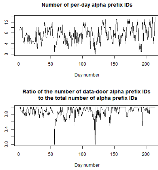
Fig. 14: A measure of the ratio of \alpha prefix IDs from/to data doors
