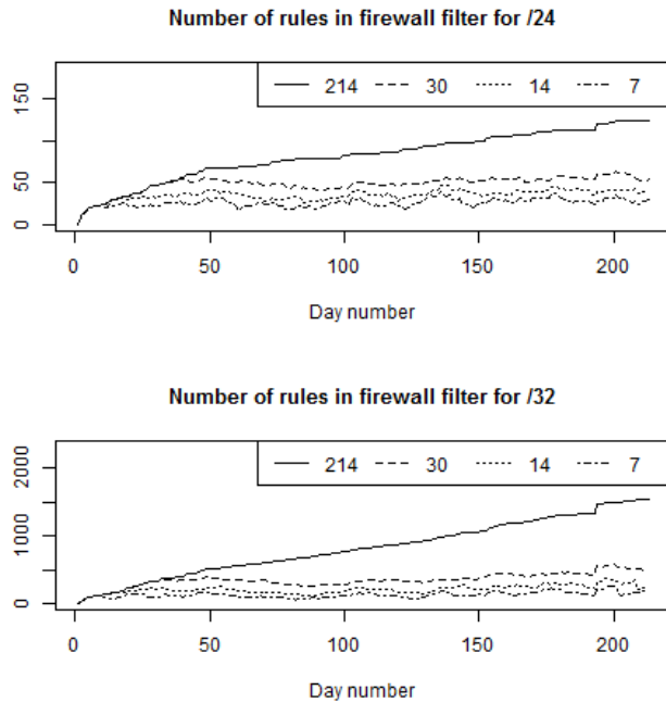
Fig. 11: Growth of firewall filter for different values of the aging parameter [6]
