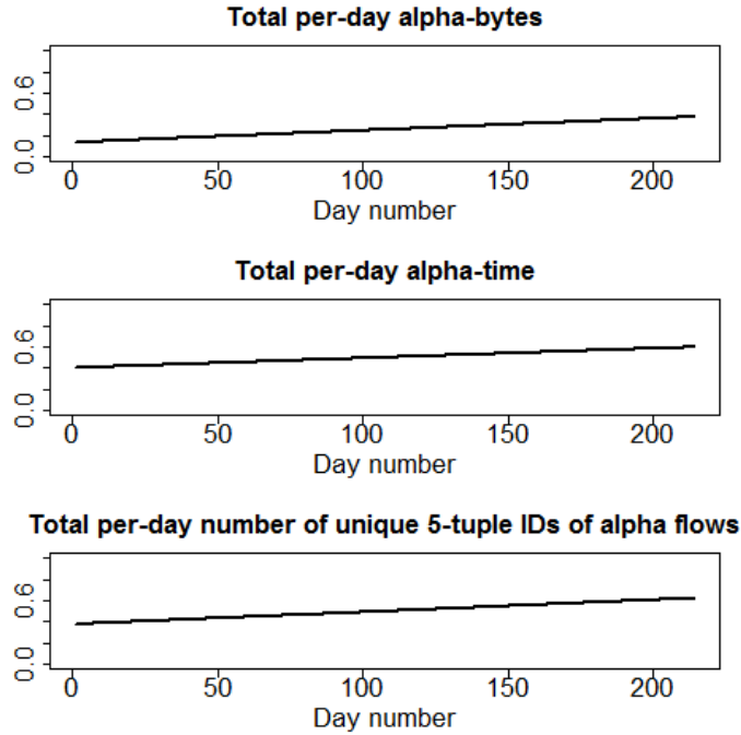
Fig. 6: Binary quantized cumulative data plus a smoothing spline function with df=2
