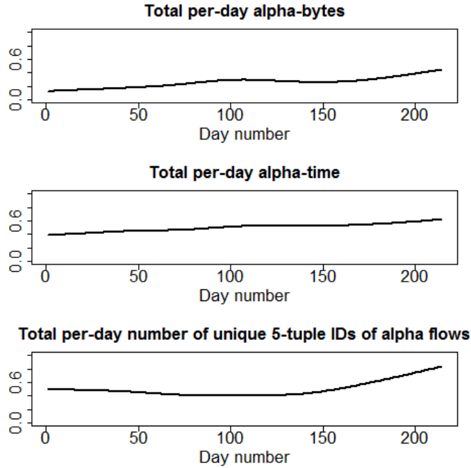
Fig. 7: Binary quantized cumulative data plus a smoothing spline function with df=4
