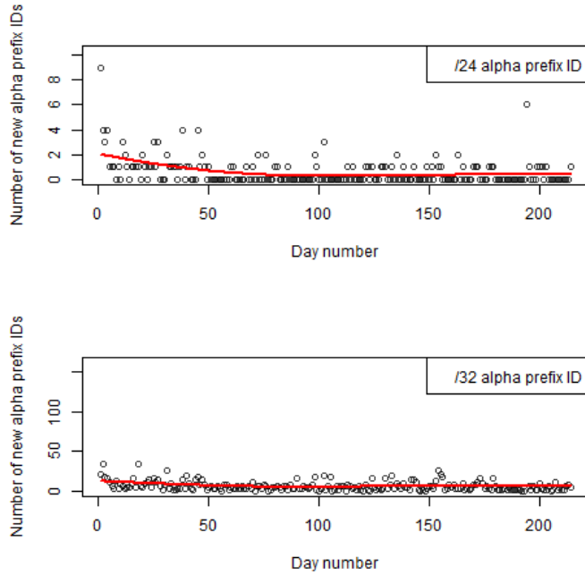
Fig. 9: Number of new \alpha prefix IDs per day with smoothing spline function (df=4)
