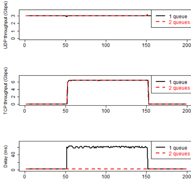
Fig. 2: The x-axis is time measured in seconds; the top graph shows that the UDP-flow rate is 3 Gbps in both the 1-queue and 2-queues configurations; the middle graph shows the TCP flow throughput; the bottom graph shows the delays experienced in the ping application [8]
