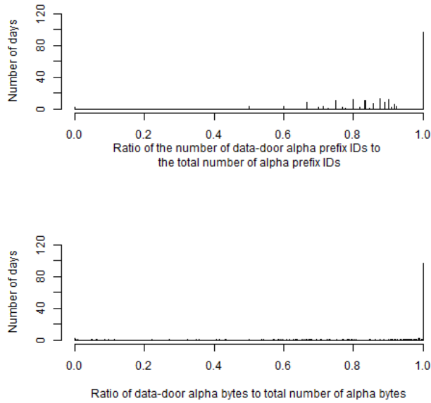
Fig. 16: Histograms of the two data-door ratio measures
