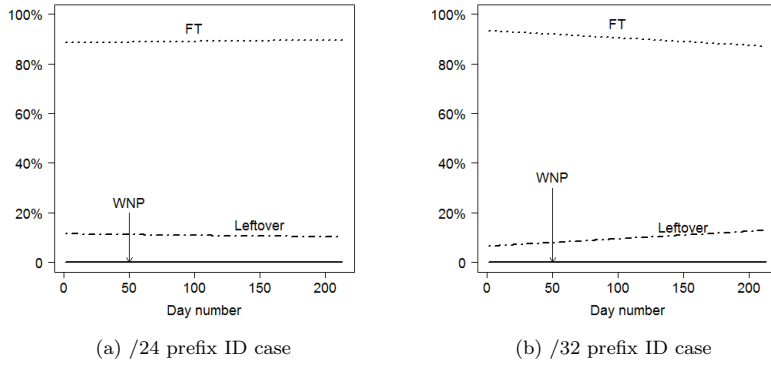
Fig. 12: Percentages of four groups of hapless \beta flow packets with smoothing spline function (df=2)
