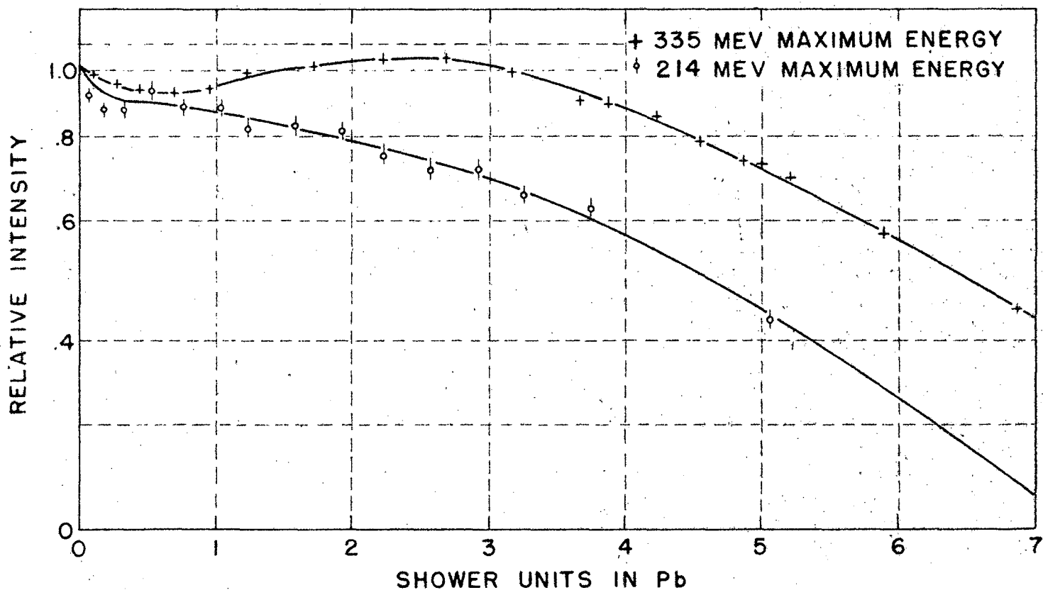
TRANSITION CURVE IN Pb OF X-RAYS CAUSING \text{C}^{12}(\gamma, n)\text{C}^{11}
