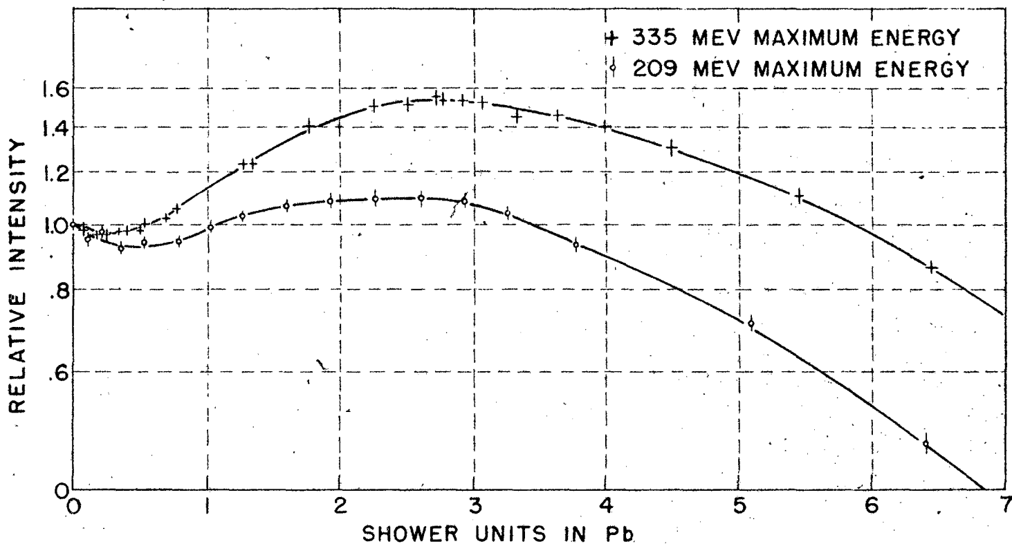
TRANSITION CURVE IN Pb OF X-RAYS CAUSING \text{Cu}^{63}(\gamma, n)\text{Cu}^{62}
