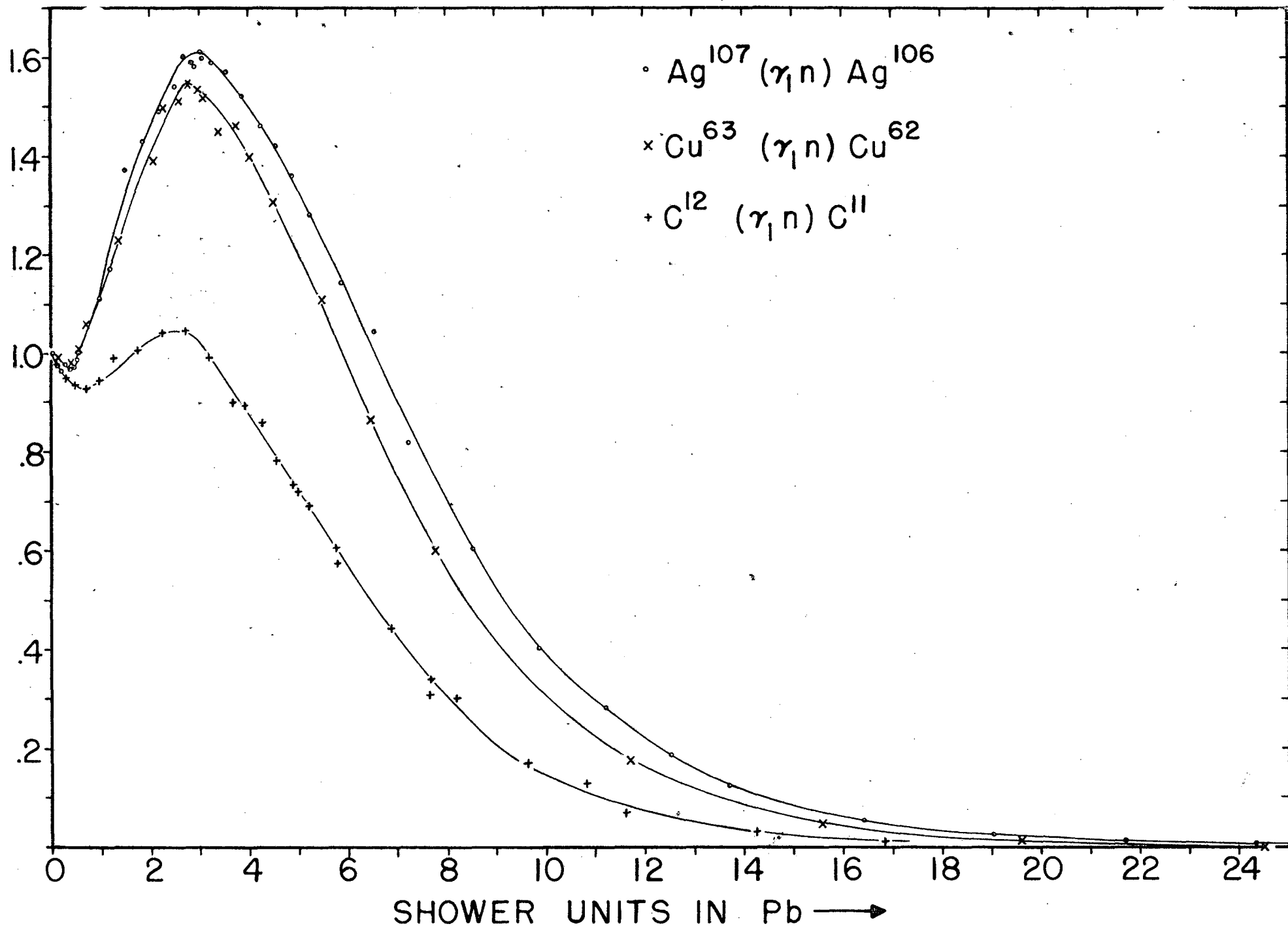
TRANSITION CURVES IN Pb OF X-RAYS CAUSING (\gamma_1 n) REACTIONS.
