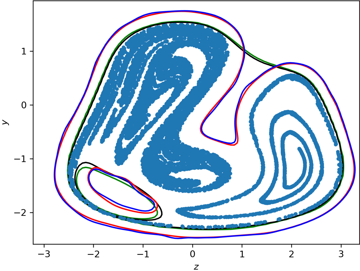
Figure 5.1: Results of Algorithms 4, 5 and 6 on the Duffing oscillator reachability problem. Black contour: output of Algorithm 4. Green contour: output of Algorithm 6. Red contour: output of Algorithm 5. Blue contour: output of Algorithm 5, over-approximated using the Nyström approximation with 1,000 samples. Blue dots: samples used in Algorithm 6.
