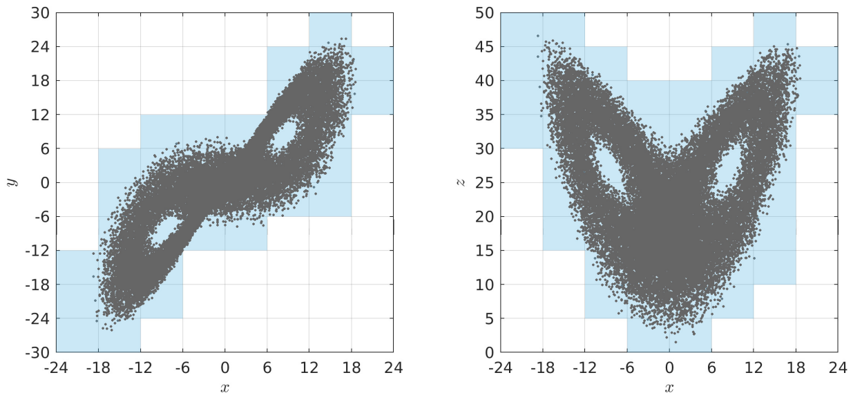
Figure 3.4: Reachable set (blue) computed by Algorithm 3 for the Lorenz system using a grid-based partition and N = 32296 samples (grey), projected onto the (x, y) and (x, z) planes.
