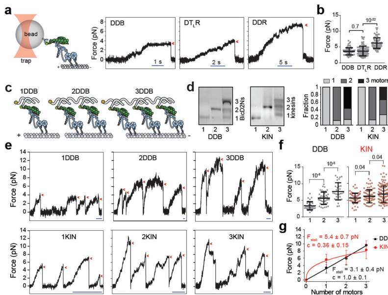
Figure 5. The multiplicity of dynein-dynactin increases total force generation. (a) (Left) Schematic of fixed optical trapping assay for measuring the stall force of single DDB tethered from the cargo adaptor (not to scale). (Right) Example traces show typical stall of a bead driven by DDB, DT L R, and DDR. The detachment of the motor from an MT after the stall is denoted by a red arrowhead. (b) Stall forces of DDB, DT L R, and DDR (mean ± s.d., n = 67 runs from 16 beads from three independent experiments for DDB, 111 runs from 24 beads from four independent experiments for DT L R, and 84 runs from 21 beads from three independent experiments for DDR). The line and whiskers represent the mean and s.d., respectively. (c) Schematic shows the assembly of 1–3 DDBs on a DNA chassis. (d) Quantification of DNA chassis labeled with 1, 2 and 3 BicD2Ns or kinesin-1 motors (right) from a native agarose gel (left) from three independent experiments. Full gels can be found at Supplementary Fig. 8. (e) Example traces show typical stalls of beads driven by single 1–3 DDB and KIN chassis in a fixed trap assay. The detachment of the motor from an MT after the stall is denoted by a red arrowhead. Scale bars are 1 s. (f) Stall forces of 1–3 DDB and 1–3 KIN chassis. From left to right, n = 35 from 12 beads, 42 from 15 beads, 32 from 10 beads, 83 from 19 beads, 72 from 17 beads and 143 from 26 beads (three independent experiments per condition). The line and whiskers represent the mean and s.d., respectively. (g) Calculated stall forces of the DNA chassis assembled with one, two and three motors after accounting for incomplete complexes (see Methods). Error bars represent s.d. Solid curves represent a fit to the power law ( y = F_{stall} \cdot x^c ) where F_{stall} is the stall force of one motor and c is the scaling exponent (mean ± s.e.). In b and g, p values are calculated using two-tailed t-test.
