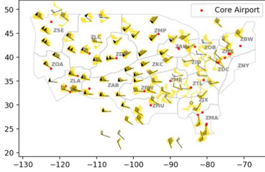
Figure 1. Wind barbs showing original winds (in yellow) and the aggregated winds (in black) at 300 hPa on 10/15/2012, 0 am – 12 pm UTC-10
