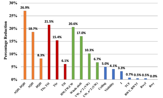
Figure 7. Relative feature importance in reducing system average delay
