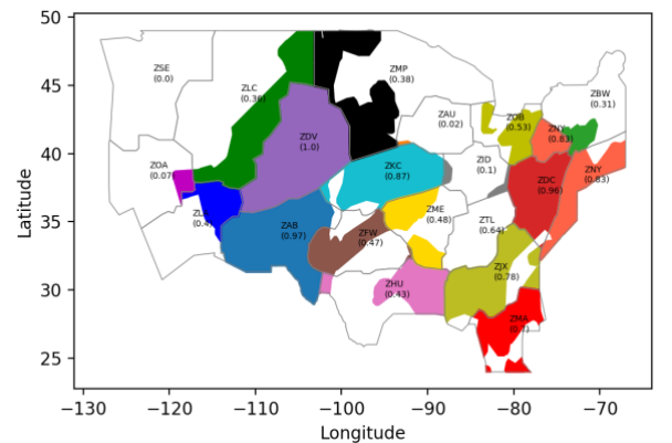
Figure 4. ARTCC-specific convection forecasts
