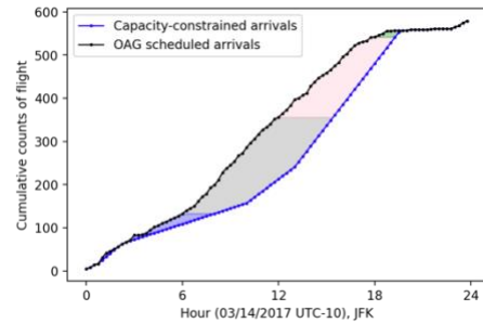
Figure 3. Queuing diagram of JFK airport on 03/14/2017 UTC-10
