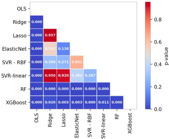
Figure 5. Heatmap showing the p -value of the model performance t -test
