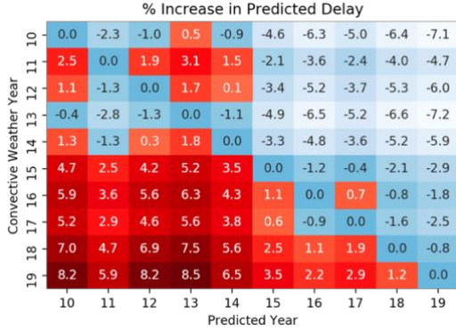
Figure 9. The all-year-pair counterfactual results for thunderstorm features
