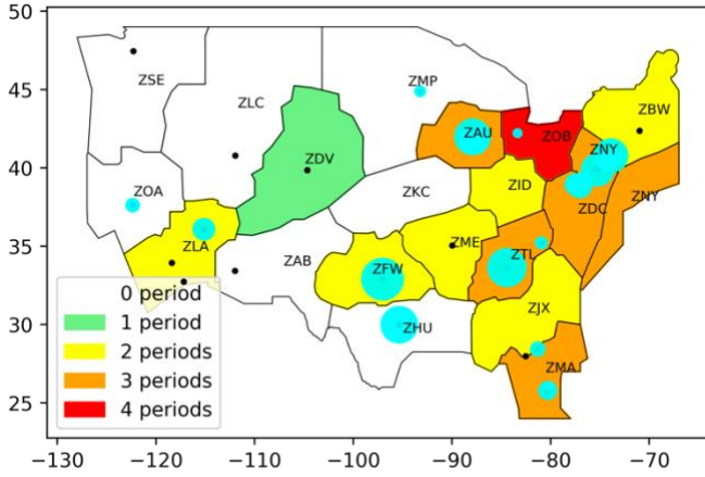
Figure 6. Spatial variability and temporal consistency of thunderstorm features and its importance to the system average arrival delay
