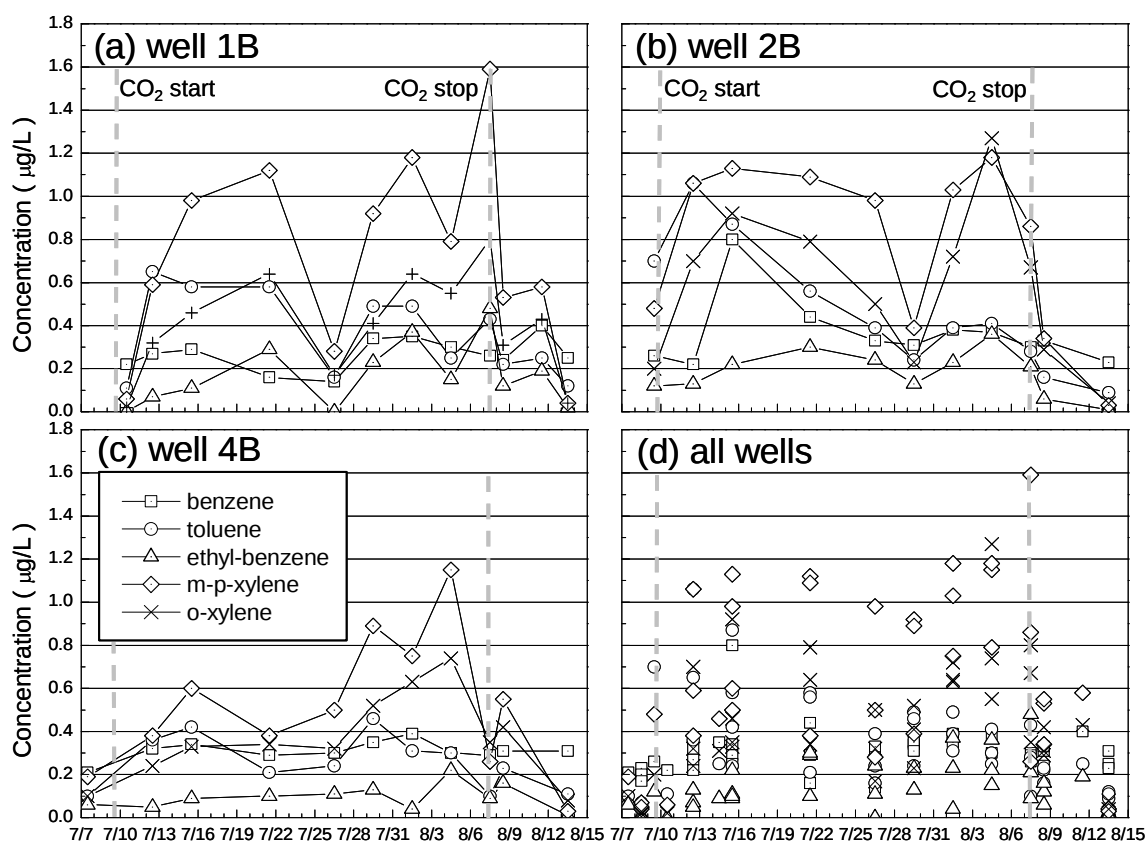
Fig. 9 Concentrations of BTEX compounds detected in groundwater from selected ZERT wells plotted as a function of time of sampling. The BTEX concentrations are all significantly below the maximum contaminant levels (MCLs) (e.g., 5 ppb for benzene). The source of the low amounts of BTEX compounds detected in groundwater following \text{CO}_2 injection is being investigated.
