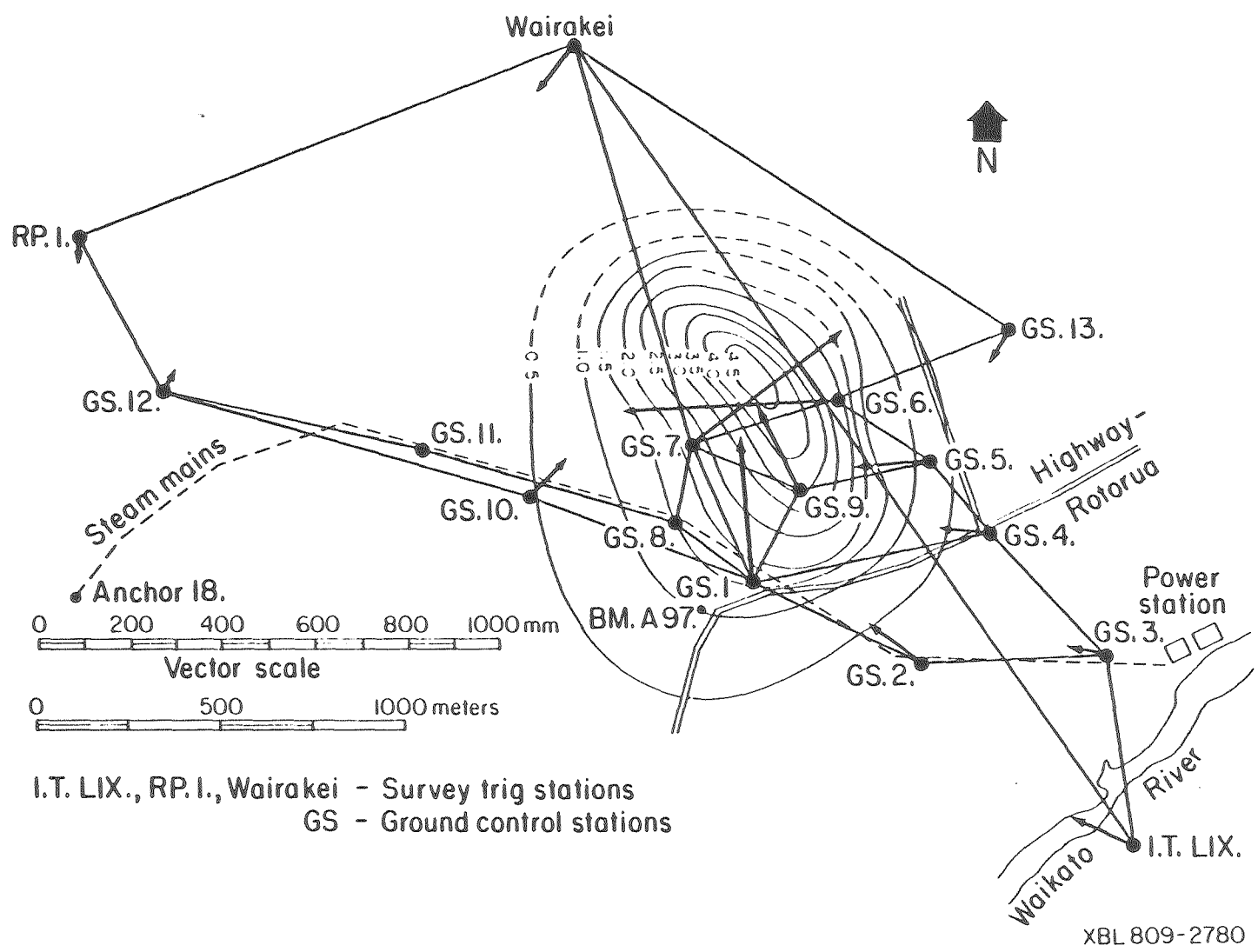
Figure 3. Horizontal displacements due to geothermal fluid withdrawal at Wairakei, New Zealand, 1964-1975 (after Stillwell et al., 1975).
