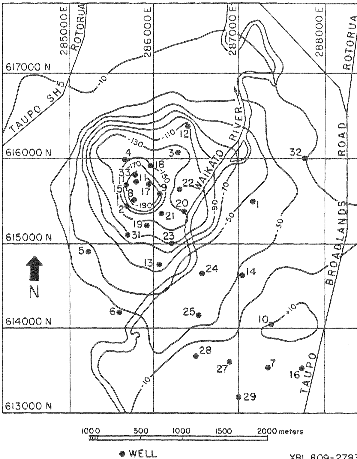
Figure 6. Subsidence at the Broadlands geothermal field between May 1968 and March 1974. Contour values are in mm. (from Ministry of Works and Development, 1977).
