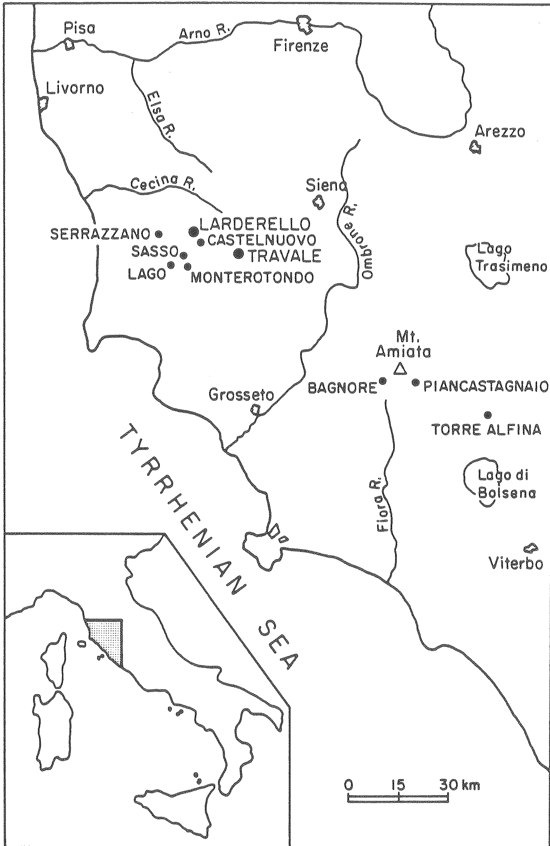
Figure 15. Location map of the Larderello geothermal field, Italy (from Atkinson et al., 1977).
