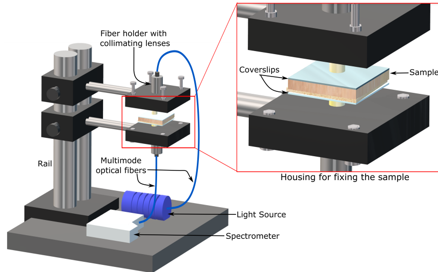
Fig. 1. Collimated transmittance measurements setup. The inset shows the housing for fixing the sample, i.e., the fiber holders with the VIS-NIR collimating lenses. As seen in the inset, the samples are placed between coverslips (see text for further details).
