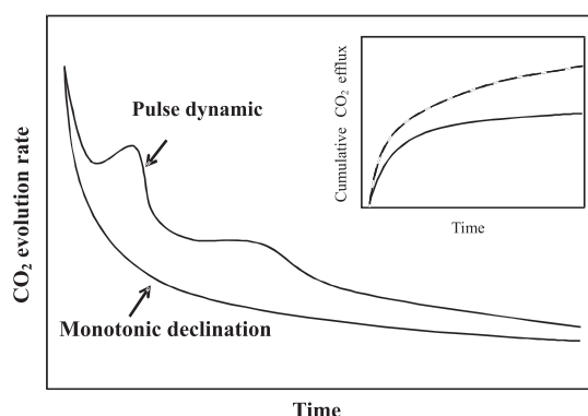
Fig. 1. Conceptual models of SOC decomposition: Commonly used models of fixed-pools with first-order kinetics predicts that soil CO 2 evolution rate from a soil incubation experiment with time would follow a pattern of monotonic decline; whereas a model based on information from studies of priming effect and other evidence would predicts that the CO 2 evolution rate would show a pattern of pulse-like fluctuations-or a pulse dynamic pattern. In the insert graph, the dashed line shows the cumulative CO 2 efflux with the pulse-dynamic pattern of soil respiration, and the solid line shows the cumulative CO 2 efflux with the monotonic decline pattern of soil respiration. Pulse dynamic patterns can be obscured if soil respiration is given as cumulative CO 2 efflux through time.
