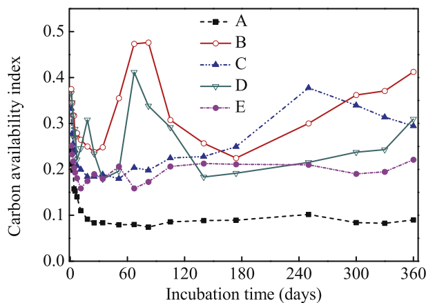
Fig. 3. The dynamics of carbon availability index (CAI) through incubation time. The overall ANOVA standard error for soils A, B, C, D and E is 0.001, 0.003, 0.002, 0.007 and 0.001, respectively. The basal respiration rate divided by the substrate induced respiration rate of each soil sample was defined as carbon availability index.
