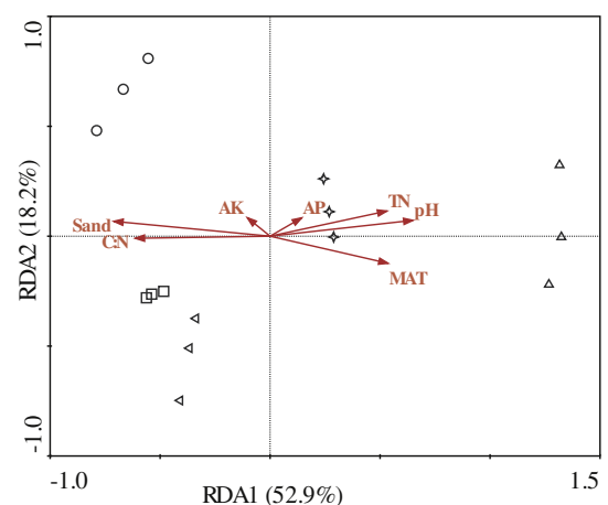
Fig. 5. Redundancy analysis (RDA) of soil respiration data and seven environment variables. Up-triangle, square, star, left-triangle and circle represents the soil taken from Pinus koraiensis and broadleaf mixed forest, Picea and Abies forest, Larix and Abies forest, Betula ermanii forest, and alpine tundra, respectively. Environmental variables are scaled by the solid axes. TN: total nitrogen; MAT: mean annual air temperature; AP: soil available phosphorous; AK: soil available potassium.
