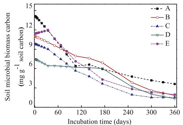
Fig. 4. The dynamics of soil microbial biomass carbon ( \text{mg g}^{-1} soil carbon) through incubation time. The overall ANOVA standard error for soils A, B, C, D and E is 0.068, 0.231, 0.077, 0.048 and 0.059, respectively.
