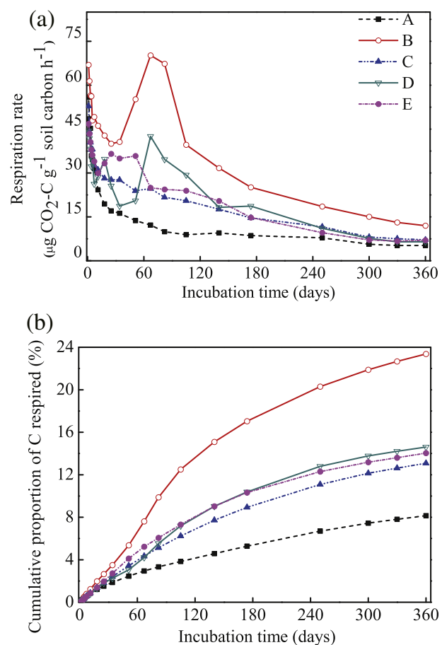
Fig. 2. Respiration rates (a) ( \mu\text{g CO}_2\text{-C g}^{-1} soil carbon \text{h}^{-1} ) and cumulative respired carbon (b) of soil samples from different elevations (A, B, C, D, and E) through incubation time. Each point in the plot represents the mean of 3 replicates ( n = 3 ). The overall ANOVA standard error for soils A, B, C, D and E is 0.161, 0.400, 0.263, 0.699 and 0.206, respectively. A, B, C, D and E represents soils taken from Pinus koraiensis and broadleaf mixed forest, Picea and Abies forest, Larix and Abies forest, Betula ermanii forest, and alpine tundra, respectively.
