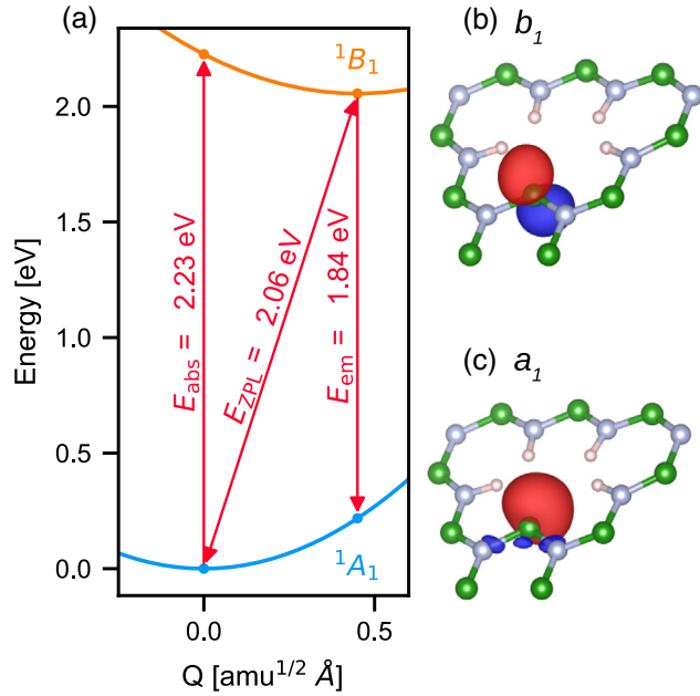
FIG. 1. (a) Calculated configuration coordinate diagram for the ^1A_1 \rightarrow ^1B_1 internal transition of the doubly occupied B DB. (b) Charge density isosurface of the B p_z state that becomes localized upon excitation. (c) Charge density isosurface of the B DB state that the electron occupies in the ground state. The isosurfaces correspond to 10% of the maximal charge density and are colored by the sign of the wave function, with red and blue indicating opposite signs.
