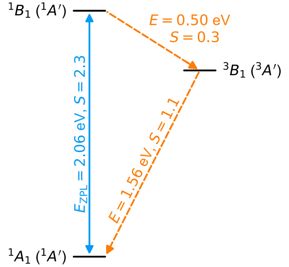
FIG. 4. Intersystem crossing of the doubly occupied B DB. The solid blue line indicates an optical transition, and dashed orange lines indicate nonradiative crossings between spin channels. Alternative labels under C_s symmetry are given in parentheses. Each transition is labeled with the transition energy and the Huang-Rhys factor S .
