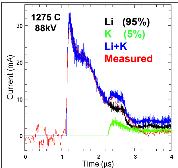
Figure 5: Measured and modeled beam current waveforms at the injector exit.
