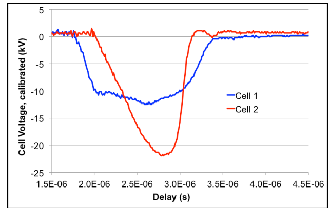
Figure 7: Voltage waveforms of induction cells 1 and 2.
