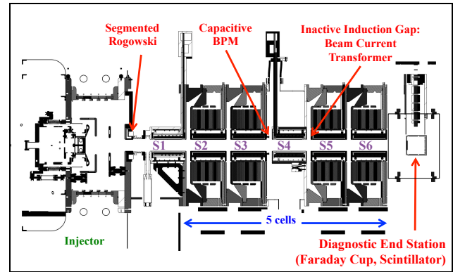
Figure 6: Injector and 5-cell beamline.
