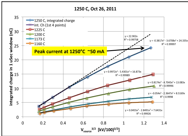
Figure 4: Measured variations in collected beam charge over 1 μsec duration.
