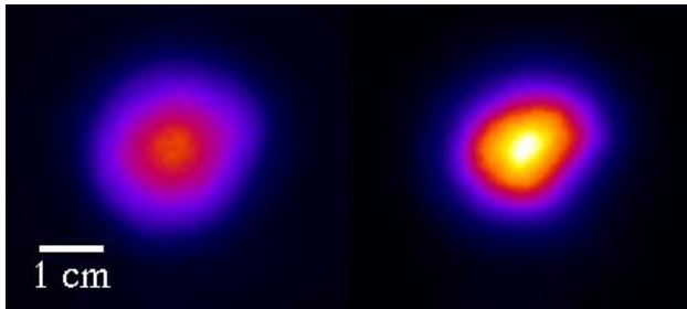
Figure 9: Beam image at injector voltage 112kV. Left: after 5-cell transport only. Right: after 5-cell transport and acceleration by 2 induction cells.
