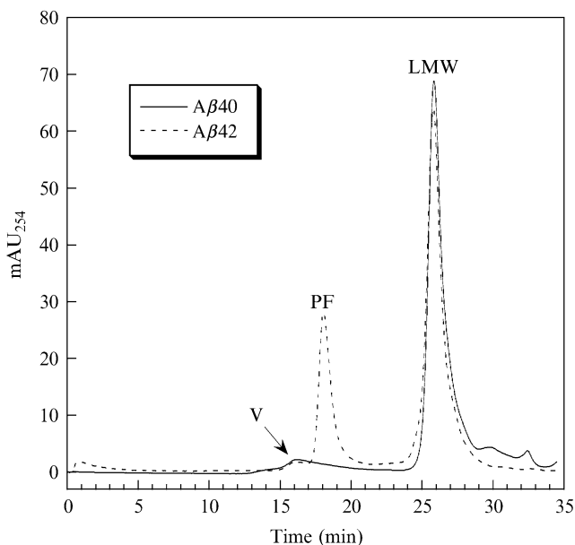
FIG. 1. Preparation of low molecular weight (LMW) amyloid \beta -protein ( A\beta ) by size exclusion chromatography (SEC). A\beta_{40} (solid line) and A\beta_{42} (dotted line) were fractionated by SEC using a Superdex 75 matrix and 10 mM sodium phosphate, pH 7.4, as the mobile phase. A small void volume peak (V) is observed in both samples, as is a major peak (LMW) in the included volume, which corresponds to LMW A\beta . A protofibril peak (PF) is shown in the A\beta_{42} sample. Adapted and reproduced with permission from Bitan et al. (2003).
