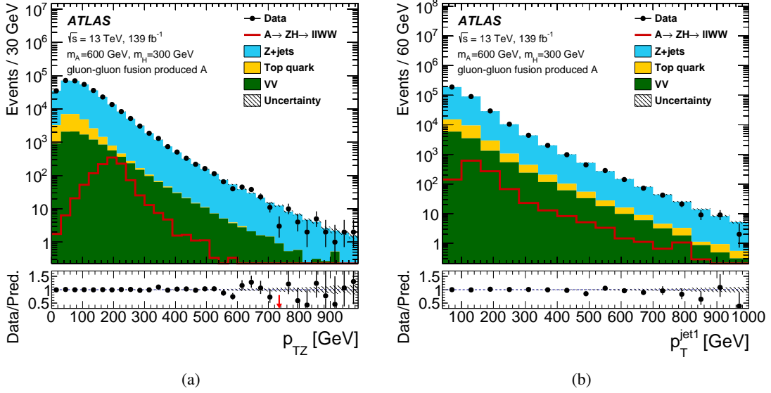
Figure 5: The distributions of (a) the p_T of the Z boson candidates and (b) the leading jet's p_T in the \ell\ell WW channel. The events are required to satisfy all the signal region criteria with the exception of the m_{4q} window requirement. Data-driven corrections are applied, as described in the text. The same conventions as in Figure 4 are used.
