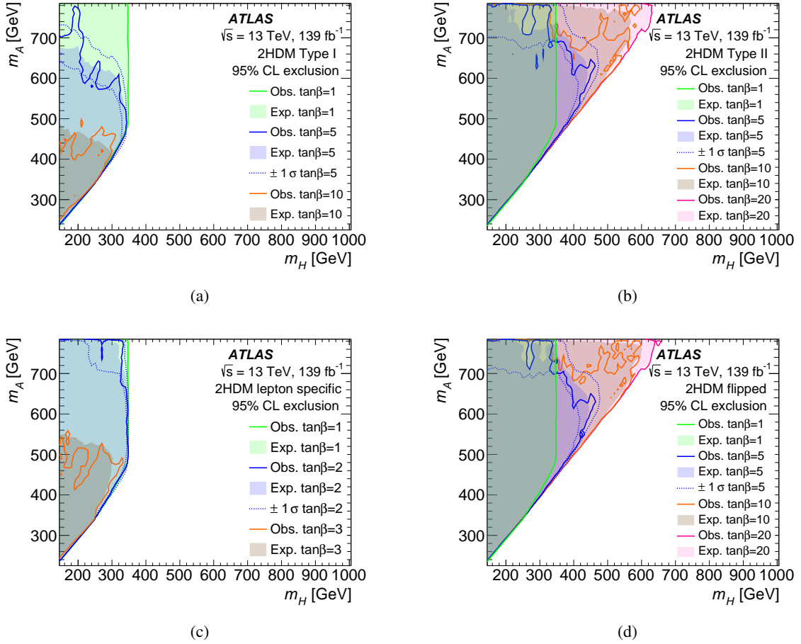
Figure 10: Observed and expected 95% CL exclusion regions for the \ell\ell b\bar{b} channel in the (m_H, m_A) plane for various \tan\beta values for the (a) type-I, (b) type-II, (c) lepton-specific and (d) flipped 2HDM, with \cos(\beta - \alpha) = 0 .
