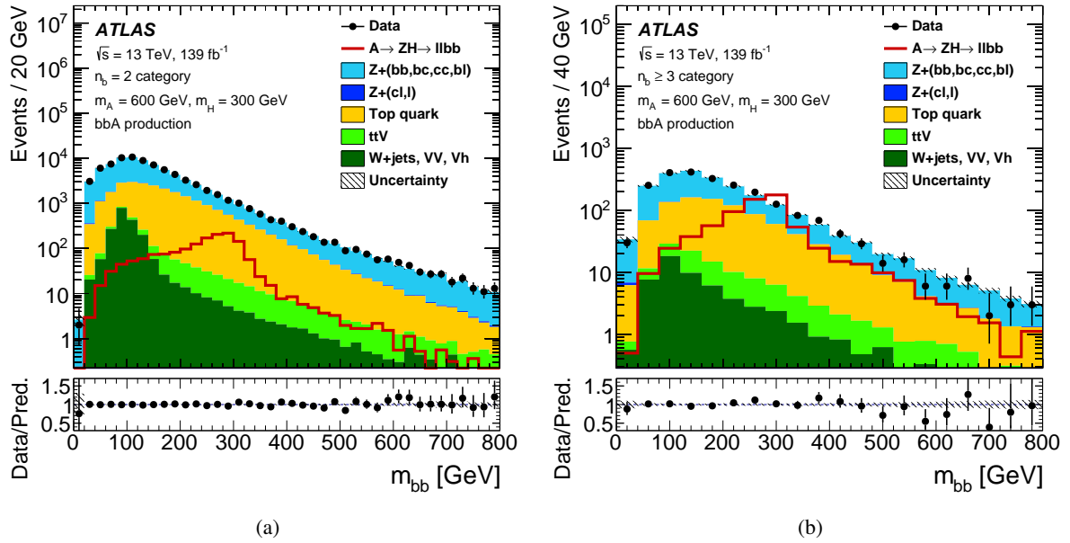
Figure 7: The m_{bb} distribution before any m_{bb} window cuts for the (a) n_b = 2 and (b) n_b \geq 3 categories. The signal distribution for (m_A, m_H) = (600, 300) GeV is also shown, and is normalised such that the production cross section times the branching ratios B(A \rightarrow ZH) and B(H \rightarrow bb) corresponds to 1 pb. The same conventions as in Figure 2 are used.
