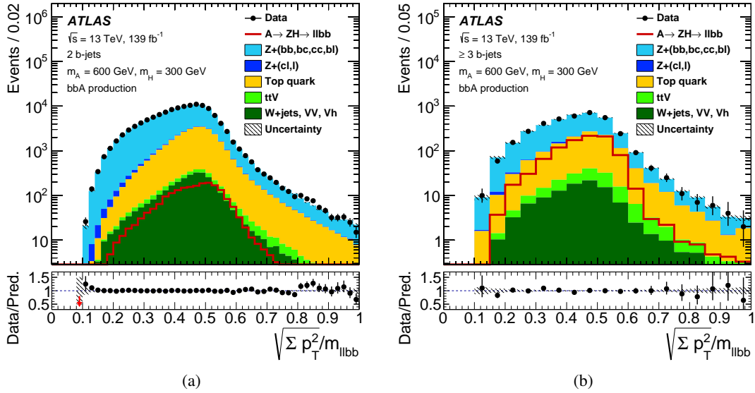
Figure 2: The \sqrt{\sum p_T^2 / m_{\ell\ell bb}} distributions shown before the requirement on this variable is applied for events with (a) exactly two b -jets and (b) three or more b -jets. Corrections from a fit to the data are applied to the simulation, as described in Sections 5.1 and 8. The signal distribution for (m_A, m_H) = (600, 300) GeV is also shown, and is normalised such that the production cross section times the branching ratios B(A \rightarrow ZH) and B(H \rightarrow bb) corresponds to 1 pb. The signal shown includes only A bosons produced in association with b -quarks. The lower panel shows the ratio of the data to the background prediction (black filled circles) and the relative uncertainty, which includes both statistical and systematic components, in the background prediction (hatched area). The notations ttV , VV and Vh refer to top-pair production in association with a vector boson, diboson production and SM Higgs boson production in association with a vector boson, respectively. The production of a Z boson in association with jets is split based on jet flavour. The notation Z+(bb, bc, cc, bl) refers to the case where the jets originate from heavy flavour, which includes at least one jet originating from a b -quark or two jets originating from c -quarks, whereas the notation Z+(cl, l) includes all the remaining cases.
