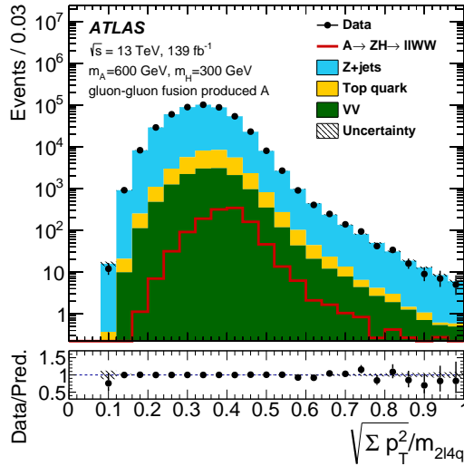
Figure 4: The \sqrt{\sum p_T^2}/m_{2\ell 4q} distribution shown before the requirement on this variable is applied. Corrections from a fit to the data are applied to the simulation, as described in Sections 5.2 and 8. The notation VV in the legend corresponds to the production of diboson events. The signal distribution for (m_A, m_H) = (600, 300) GeV is also shown, and is normalised such that the production cross section times the branching ratios B(A \rightarrow ZH) and B(H \rightarrow WW) corresponds to 1 pb. The lower panel shows the ratio of the data to the background prediction (black filled circles) and the relative uncertainty, which includes both statistical and systematic components, in the background prediction (dashed area).
