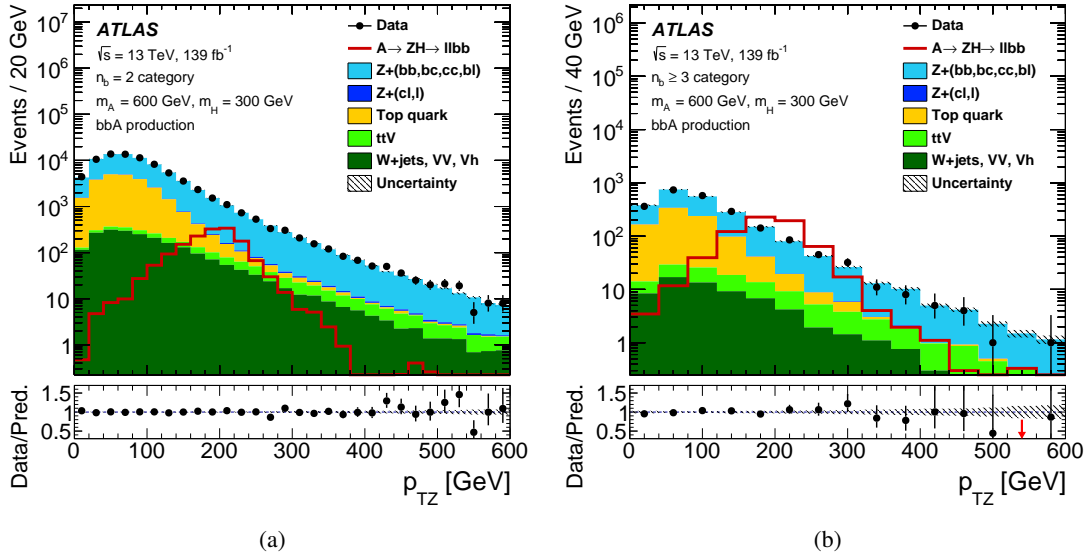
Figure 3: The p_{TZ} distributions for (a) the n_b = 2 and (b) the n_b \geq 3 category. The events are required to satisfy all the signal region criteria with the exception of the m_{bb} window requirement. The same conventions as in Figure 2 are used.
