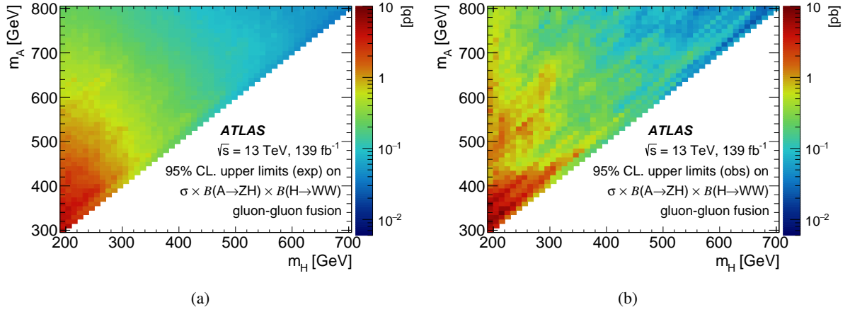
Figure 13: Expected (a) and observed (b) upper bounds at 95% CL on the production cross section times the branching ratio B(A \rightarrow ZH) \times B(H \rightarrow WW) in pb.
