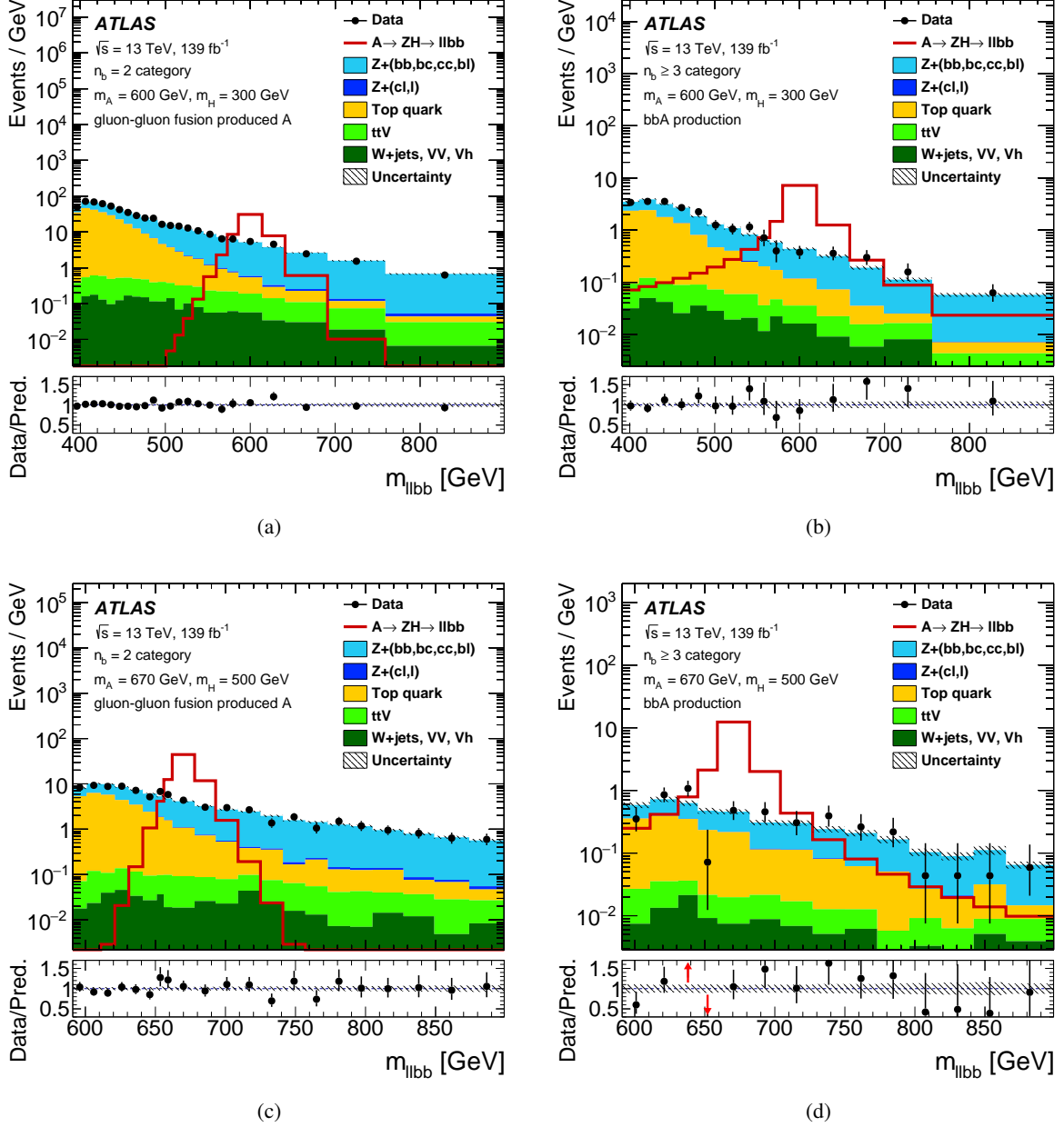
Figure 8: The m_{\ell\ell b b} mass distribution for the m_{bb} windows defined for m_H = 300 GeV and m_H = 500 GeV for (a, c) the n_b = 2 and (b, d) the n_b \geq 3 category, respectively. Signal distributions with (m_A, m_H) = (600, 300) GeV and (m_A, m_H) = (670, 500) GeV are also shown for gluon-gluon fusion production in (a, c) and b -associated production in (b, d). The number of entries shown in each bin is the number of events in that bin divided by the width of the bin. The same conventions as in Figure 2 are used.
