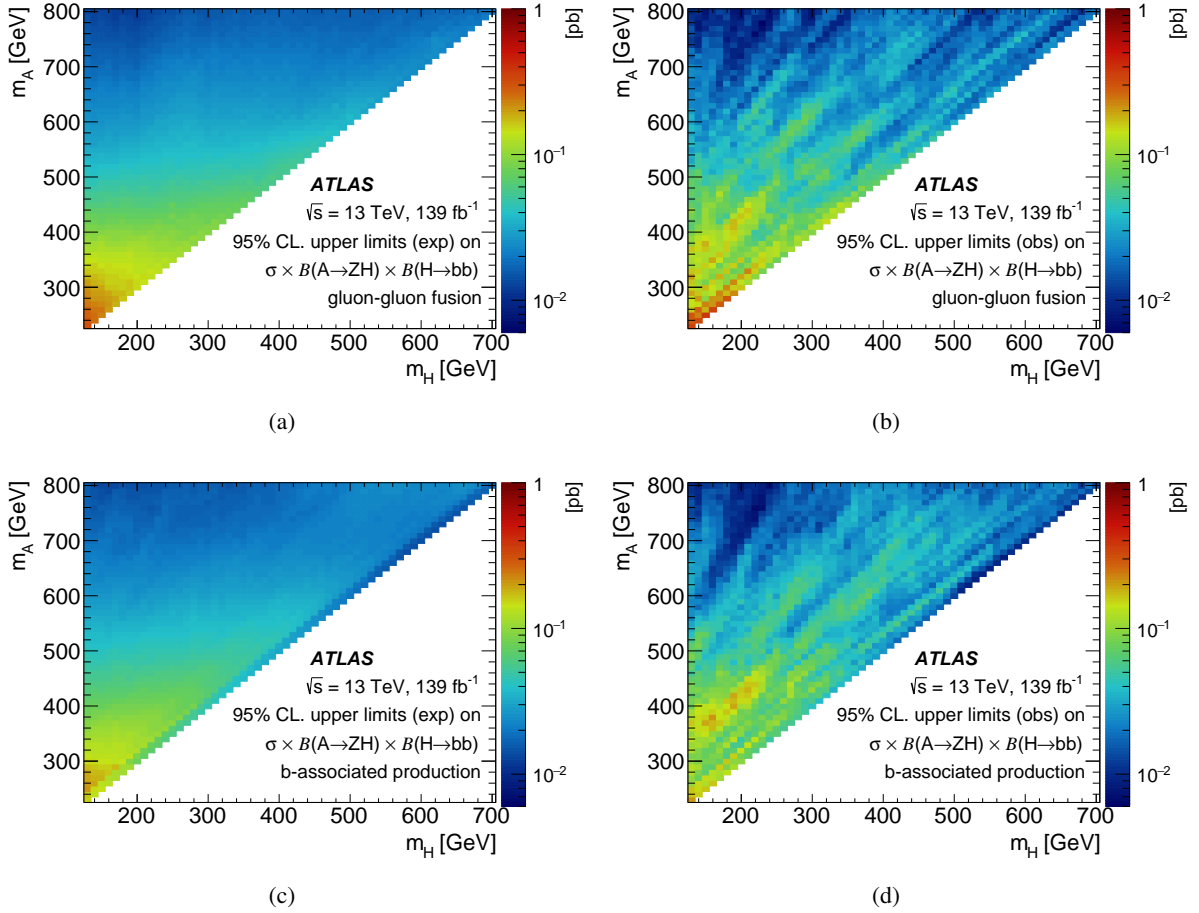
Figure 9: Upper bounds at 95% CL on the production cross section times the branching ratio B(A \rightarrow ZH) \times B(H \rightarrow bb) in pb for (a, b) gluon–gluon fusion and (c, d) b -associated production. The expected upper limits are shown in (a) and (c) and the observed upper limits are shown in (b) and (d).
