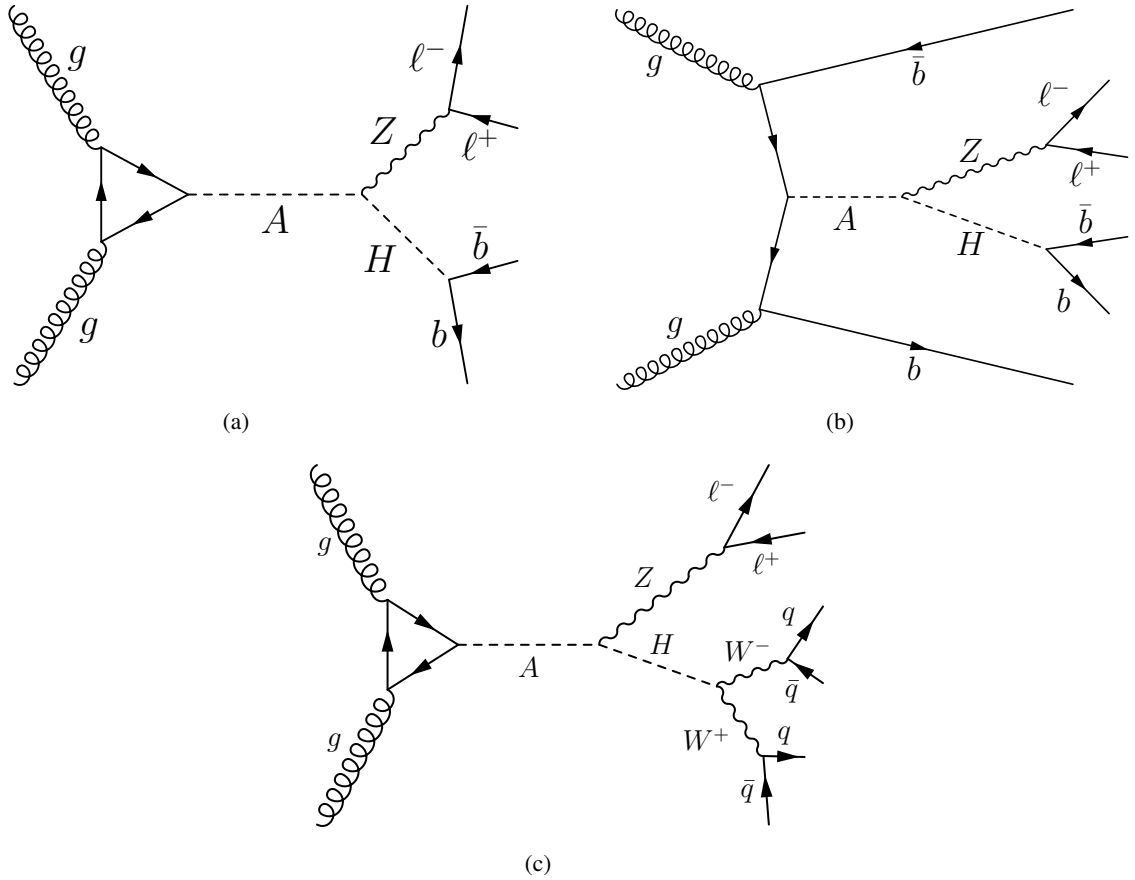
Figure 1: Example lowest-order Feynman diagrams for (a) gluon–gluon fusion production of A bosons decaying into ZH \rightarrow \ell\ell b\bar{b} , (b) b -associated production of A bosons decaying into ZH \rightarrow \ell\ell b\bar{b} , and (c) gluon–gluon fusion production of A boson decaying into ZH \rightarrow \ell\ell WW .
