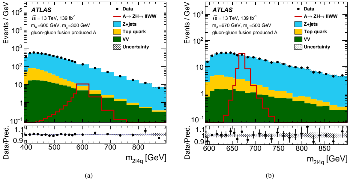
Figure 12: The m_{2\ell 4q} mass distribution for the m_{4q} windows defined for (a) m_H = 300 GeV and (b) m_H = 500 GeV. Signal distributions are also shown with (m_A, m_H) = (600, 300) GeV and (m_A, m_H) = (670, 500) GeV. The number of entries shown in each bin is the number of events in that bin divided by the width of the bin. The same conventions as in Figure 4 are used.
