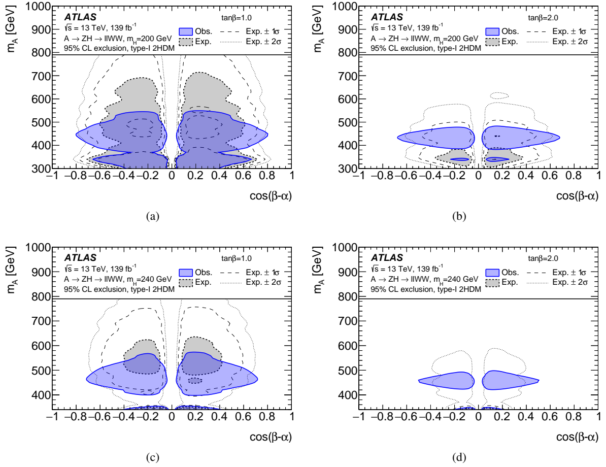
Figure 14: Observed and expected 95% CL exclusion regions in the (\cos(\beta - \alpha), m_A) plane for various \tan\beta values for (a,b) m_H = 200 GeV and (c,d) m_H = 240 GeV in the context of type-I 2HDM for the \ell\ell WW channel.
