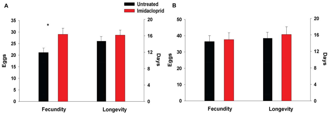
Figure 3. Effect of exposure to imidacloprid on lifetime fecundity and longevity of T. schoenei . (A) Effect of imidacloprid delivered through plant tissue. T. schoenei consuming foliage from elms treated with imidacloprid ( N=8 ) laid significantly more eggs than spider mites feeding on leaves from untreated trees ( N=8 ), while their longevity was not affected. (B) Topical application of imidacloprid to T. schoenei . Females ( N=30 ) sprayed with imidacloprid did not exhibit higher fecundity or longevity than T. schoenei sprayed with water ( N=30 ). Means \pm s.e.m. marked with asterisks are significantly different at P<0.05 . doi:10.1371/journal.pone.0020018.g003
