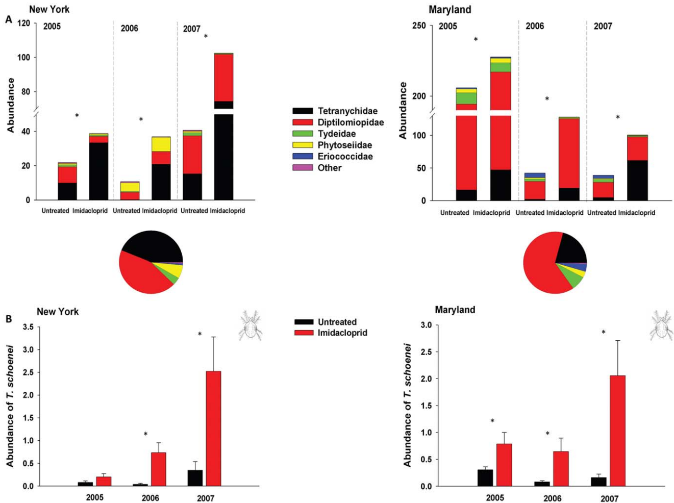
Figure 1. Effect of imidacloprid on arthropod communities and spider mite abundance in New York and Maryland. (A) Abundance of arthropods (per cm 2 of leaf area) on imidacloprid-treated elms (N=10) and on untreated trees (N=10). Asterisks mark differences in overall abundance of arthropods that were significant within each year (P<0.05; Monte Carlo permutation test). At both locations, arthropod communities increased on elms that received imidacloprid. Abundance of spider mites, Tetranychidae, explained most of the variation due to imidacloprid treatments. Pie charts represent percent contribution of the most abundant taxa to the sampled arthropod community over three-year period at each location. (B) Abundance ((number)/cm 2 ) of the spider mite, T. schoenei , on elms treated with imidacloprid (N=10) and on untreated trees (N=10) in New York and Maryland. Asterisks mark means±s.e.m. that differed significantly (P<0.05). There was a significant interactive effect of treatment and time for both locations and in most years, and means were compared within each date (Table S1). Elevated densities of mites were found only on elms treated with imidacloprid. Rarely encountered taxa included arthropods in families Chrysopidae, Coccinellidae, Cecidomyiidae, Aphididae, Saproglyphidae and Thripidae. These arthropods were pooled and categorized as ‘Other’. doi:10.1371/journal.pone.0020018.g001
