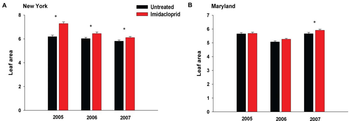
Figure 4. Effect of imidacloprid on elm leaf area in New York (A) and Maryland (B). Figure depicts area of leaves ( \text{cm}^2 ) used in surveys of arthropod community presented in Figure 1. Elms (treated: N=10 ; untreated: N=10 ) in New York had a significantly greater leaf area following exposure to imidacloprid in all sampling years, while trees in Maryland (treated: N=10 ; untreated: N=10 ) were larger in the last year of the study. Means \pm s.e.m. marked with asterisks are significantly different at P<0.05 . doi:10.1371/journal.pone.0020018.g004
