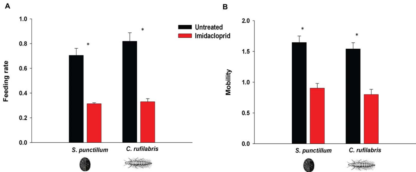
Figure 2. Feeding rate and mobility of S. punctillum and C. rufilabris exposed to imidacloprid through prey. A) Feeding rates ( \sqrt{} (mites eaten)/h) of S. punctillum and C. rufilabris were reduced after 3.5 h when mites were reared on foliage from imidacloprid-treated ( N=7 ) compared to untreated elms ( N=7 ). (B) Mobility ( \sqrt{} (mm/s) of S. punctillum and C. rufilabris was significantly reduced after 3.5 h of exposure to spider mites reared on foliage from imidacloprid-treated elms compared to untreated elms. Means \pm s.e.m. marked with asterisks are significantly different at P<0.05 . doi:10.1371/journal.pone.0020018.g002
