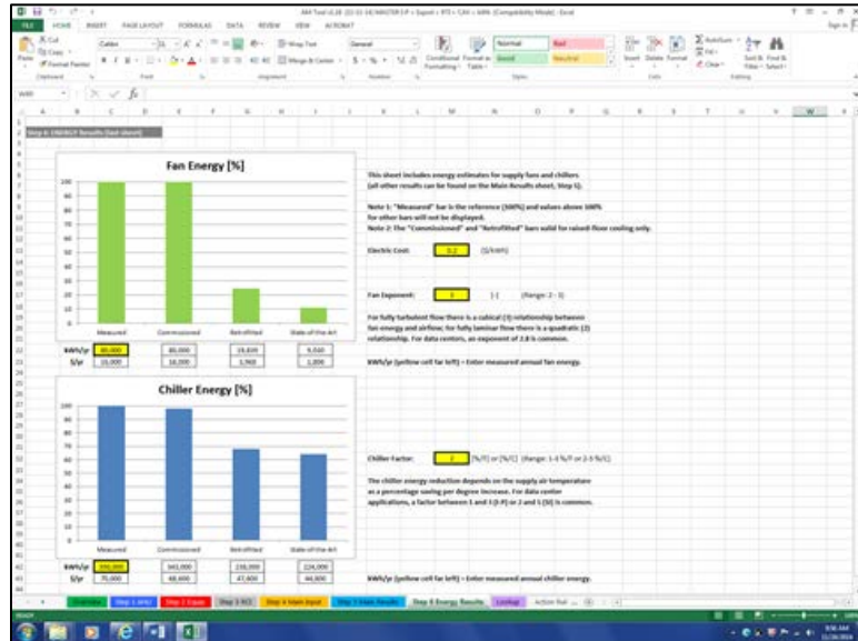
Figure 5.1.1: The Air Management Tool’s Energy Results Sheet
