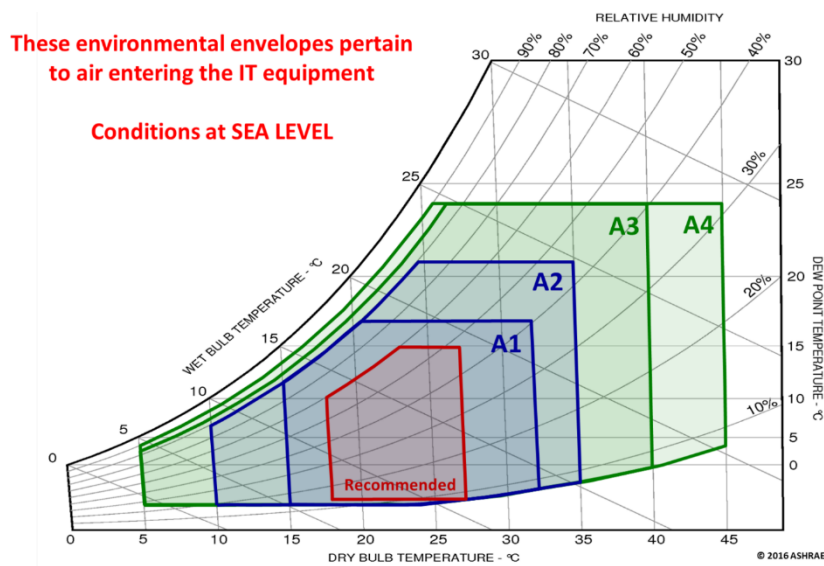
Figure 6.1: ASHRAE Recommended and Allowable Environmental Envelopes (ASHRAE 2015)
