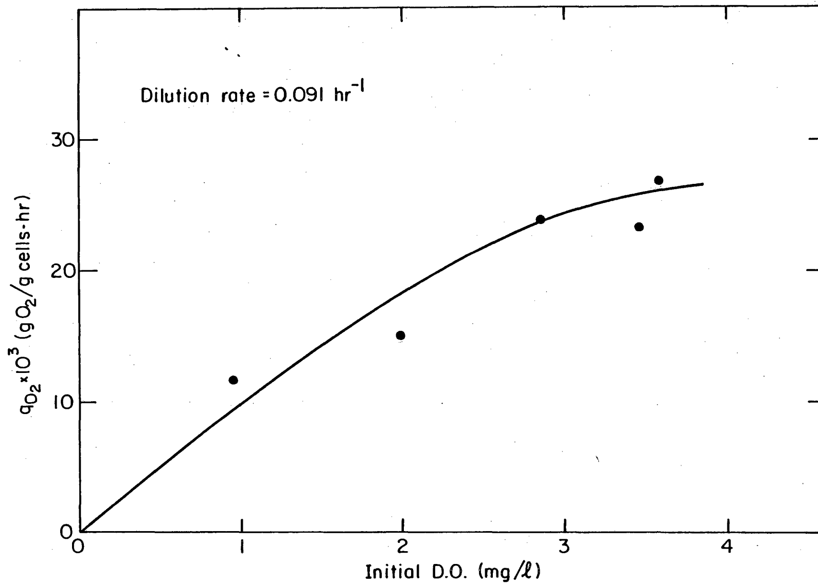
Figure IIB-3. Specific oxygen consumption versus initial dissolved oxygen at a dilution rate of 0.091/hr.
