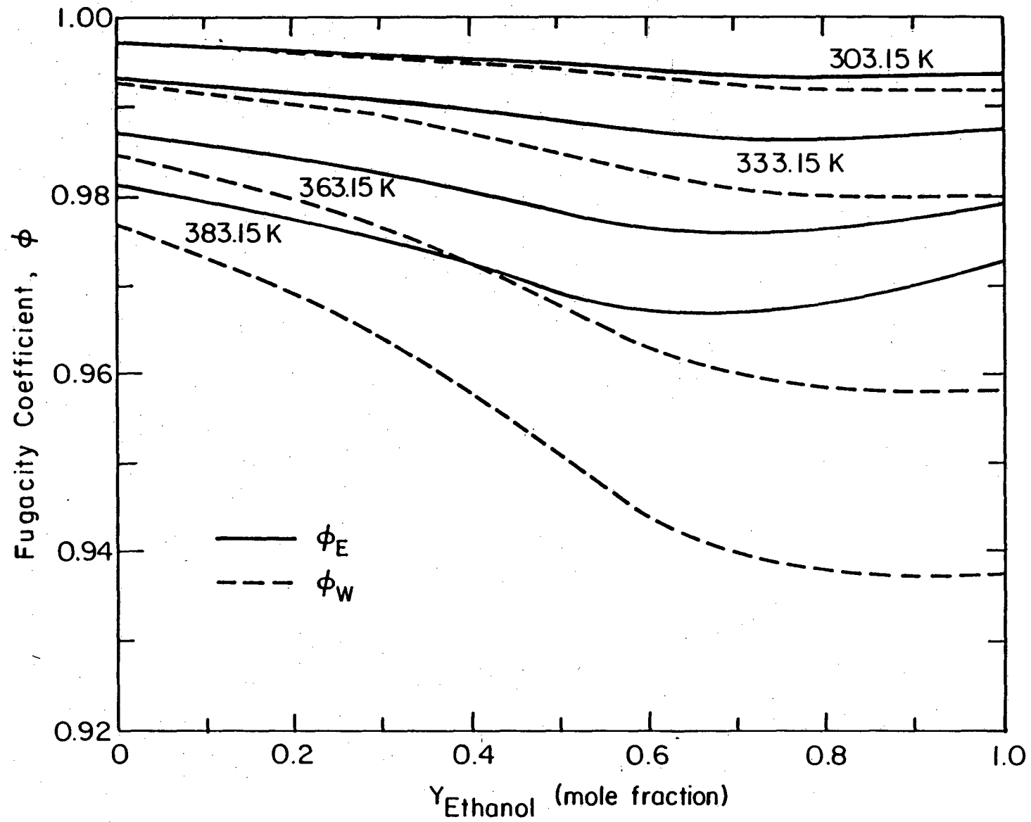
Figure IIIA-3. Fugacity coefficient at saturation pressure for specified composition at temperature.
