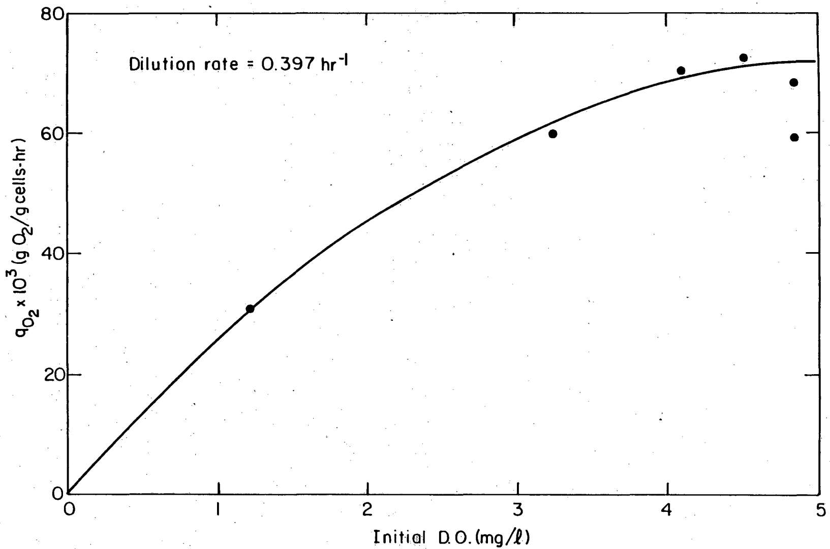
Figure IIB-8. Specific oxygen consumption versus initial dissolved oxygen at a dilution rate of 0.397/hr.
