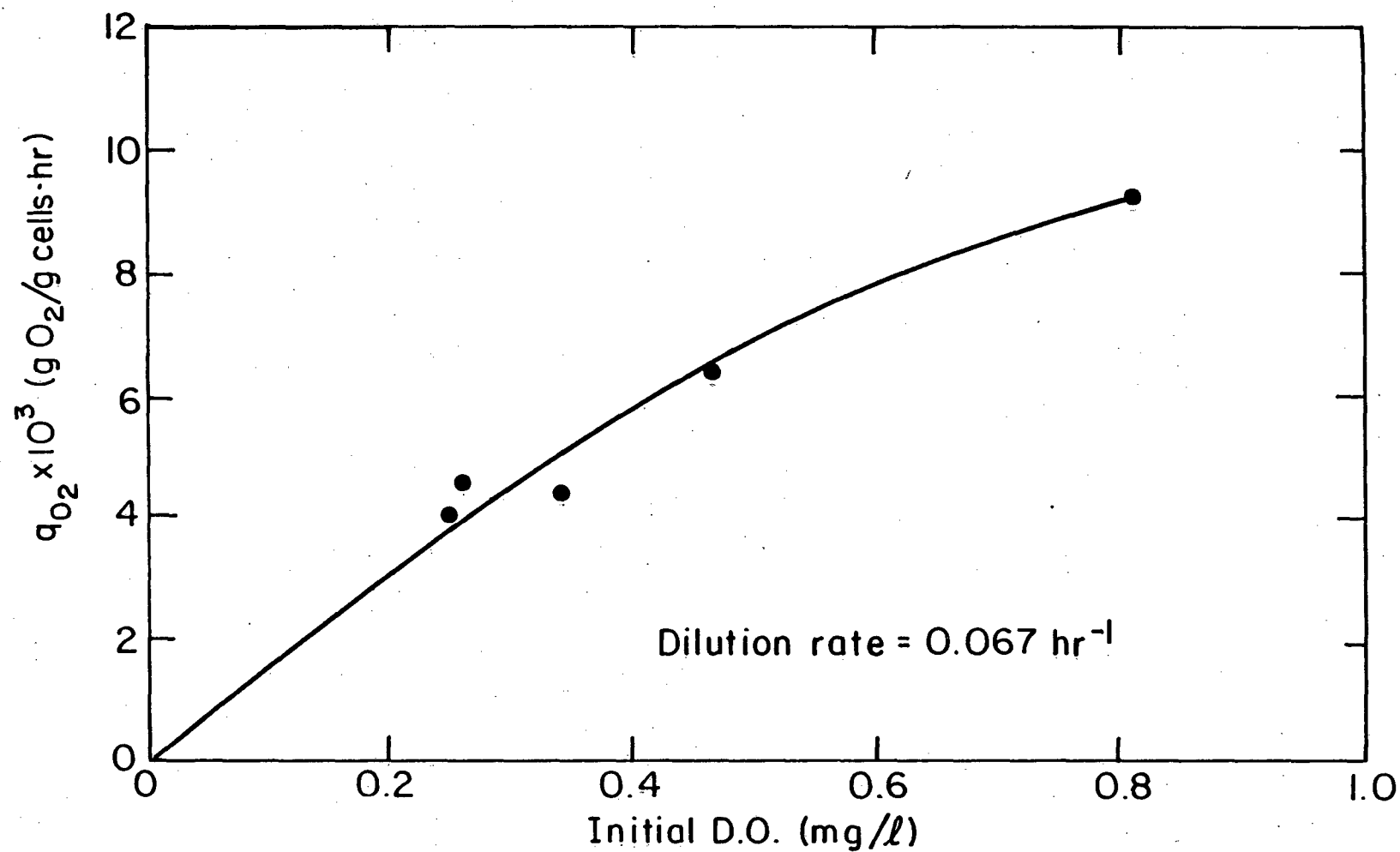
Figure IIB-2. Specific oxygen consumption versus initial dissolved oxygen at a dilution rate of 0.067/hr.
