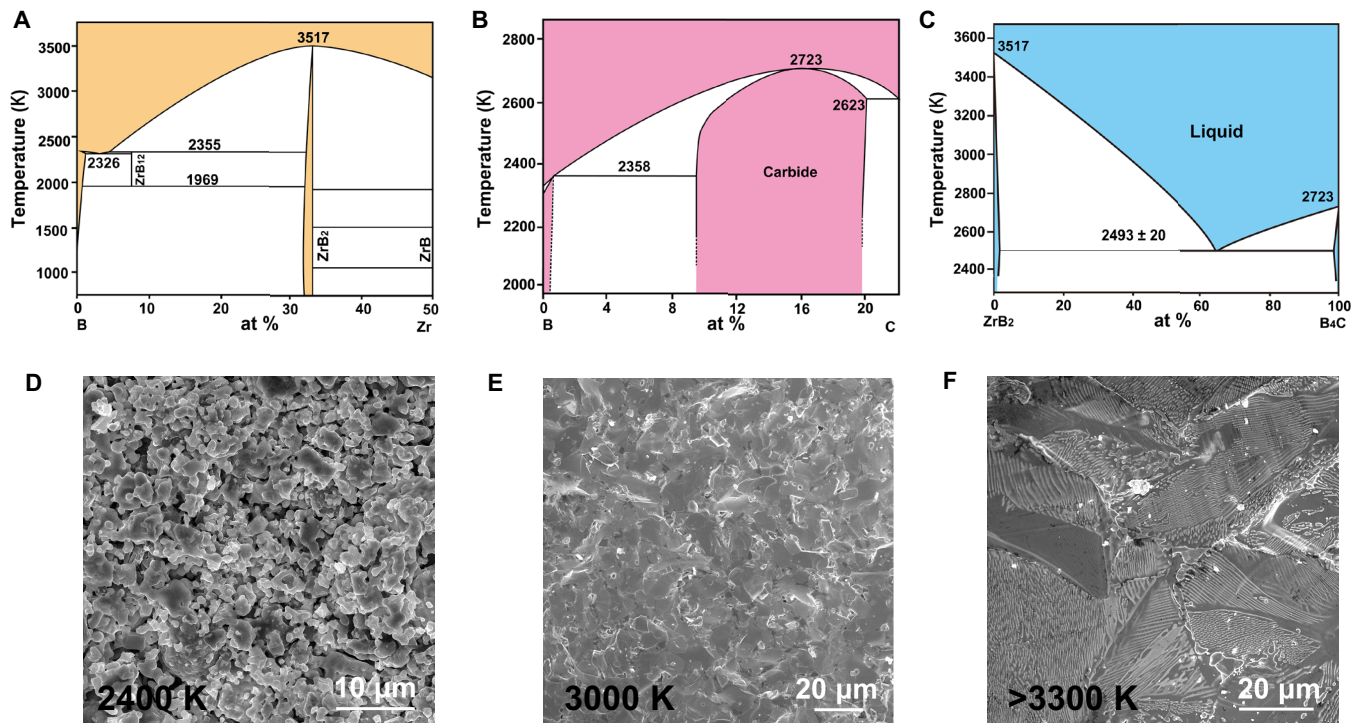
Fig. 2. The influence of temperature and phases on the sintering results. Phase diagrams of the (A) B-Zr, (B) B-C, and (C) ZrB_2 - B_4C components (36, 38, 41). At 3000 K, the high-entropy metal diborides can maintain a solid state, while the boron carbide couples with the HEB to form the eutectic liquid phase. Scanning electron microscopy (SEM) images showing the morphologies of the composite samples at different sintering temperatures of (D) 2400 K, (E) 3000 K, and (F) above 3300 K. The optimal temperature here for the rapid sintering of the HEB composite is around 3000 K. at %, atomic %.
