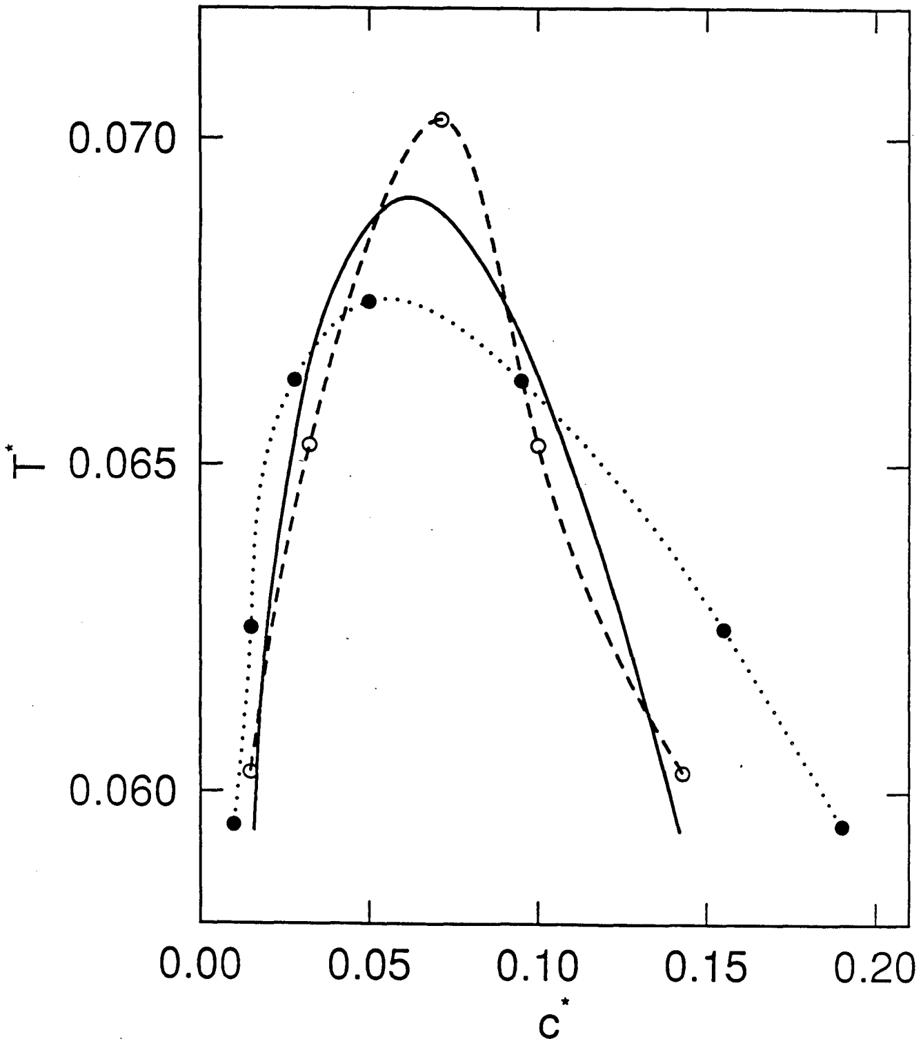
Figure 1. Vapor - liquid coexistence curve for an ionic fluid. The solid curve denotes the proposed equation of state with variables recalculated from T and V into T^* = 1/\beta^* and c^* . The solid and open circles denote the results for the restricted primitive model obtained by Schreiber and Pitzer (1987) and Valleeau (1991), respectively.
