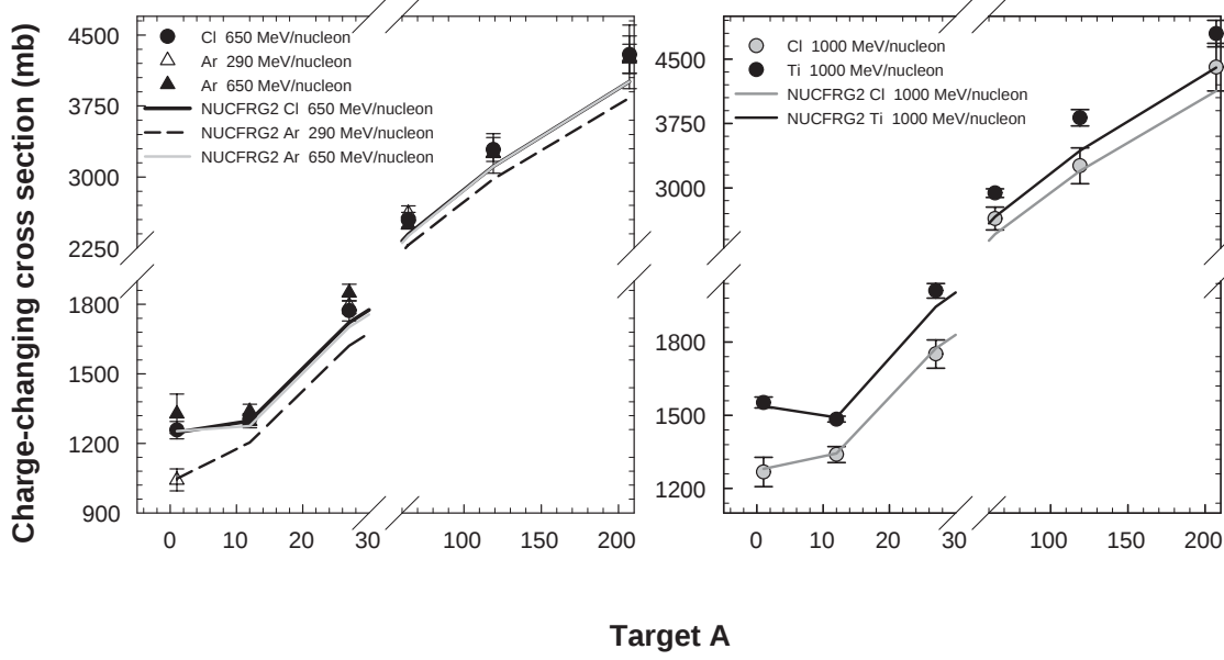
FIG. 7: Charge changing cross sections compared to NUCFRG2 predictions. In the figure on the left, results for 650 MeV/nucleon ^{35}\text{Cl} and ^{40}\text{Ar} beams are shown, along with 290 MeV/nucleon ^{40}\text{Ar} data. The figure on the right shows the results for the two 1000 MeV/nucleon beams measured here, ^{35}\text{Cl} and ^{48}\text{Ti} . In all cases the hydrogen-target data have been multiplied by a factor of 2.5 to compress the scales.
