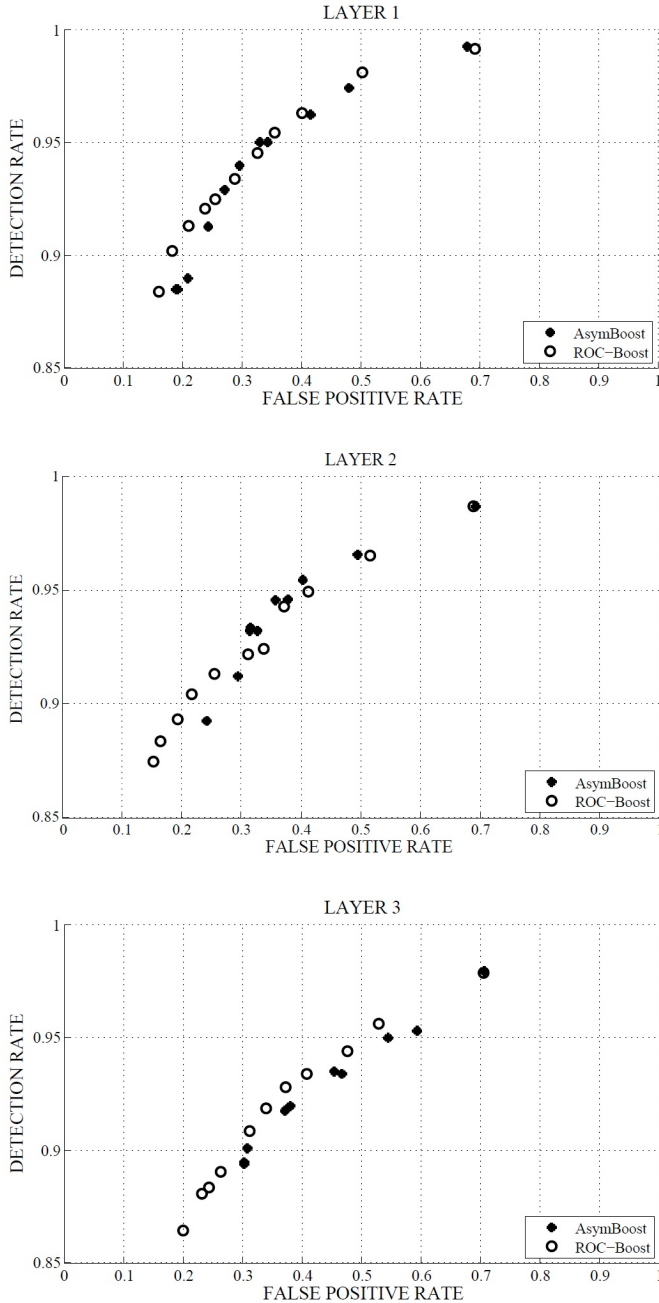
Fig. 3. Detection rate vs. false positive rates for the ROC-Boost and AsymBoost classifiers, trained on TrialTrain and tested on TrialTest (see text for details).
