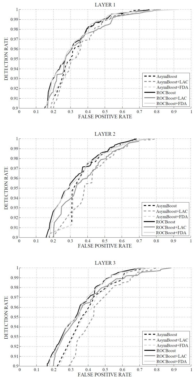
Fig. 2. The Pareto front of the ROC curves for the different classifiers considered. The Pareto fronts were computed over the ROC curves obtained by changing the value of \bar{D}_{\text{bound}} between 0.01 and 0.3 (for ROC-Boost) and of k between 2 and 5 (for Asymboost), and for multiple values of the final threshold c . The classifiers were trained and tested on the same dataset (TrialTrain).
