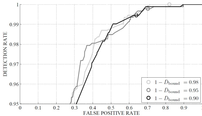
Fig. 1. ROC curves obtained from ROC-Boost classifiers, trained and tested over the whole data set with the features in Layer 1 for three different values of \bar{D}_{\text{bound}} . The circles represent the performance of the classifier produced by the ROC-Boost design algorithm; the ROC curve is obtained by varying the threshold c of the strong classifier.
