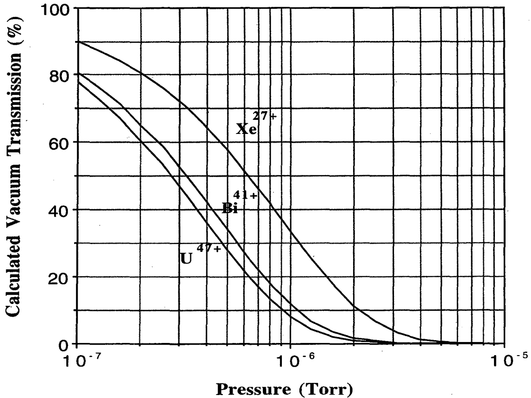
Fig. 6. Calculated beam vacuum transmission versus pressure for Xe 27+ , Bi 41+ and U 47+ ion beams accelerated by the 88-Inch Cyclotron. Improvement ratios are in good agreement with the measured data.
