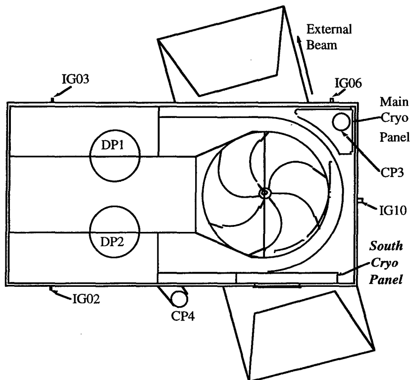
Fig. 3. A plan view of the 88-Inch Cyclotron with the current pumping layout showing the newly installed "South Cryo Panel" and ion gauge IG10 located in between the two cryo panels.
