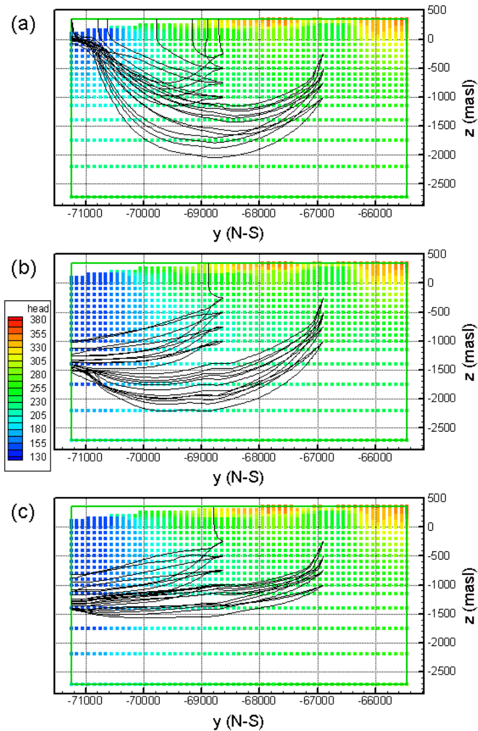
Figure 4. North-south cross-sectional (y-z) view of the streamtraces from the monitoring points. All x (E-W) values are projected on a single plane. In (a) the lateral constant-head boundaries extend less than 500 m below the ground surface; in (b) and (c) they extend over all but the lowest two layers of the model. In (c) the permeability in each of the lowest three layers is three times smaller than the permeability above it.
