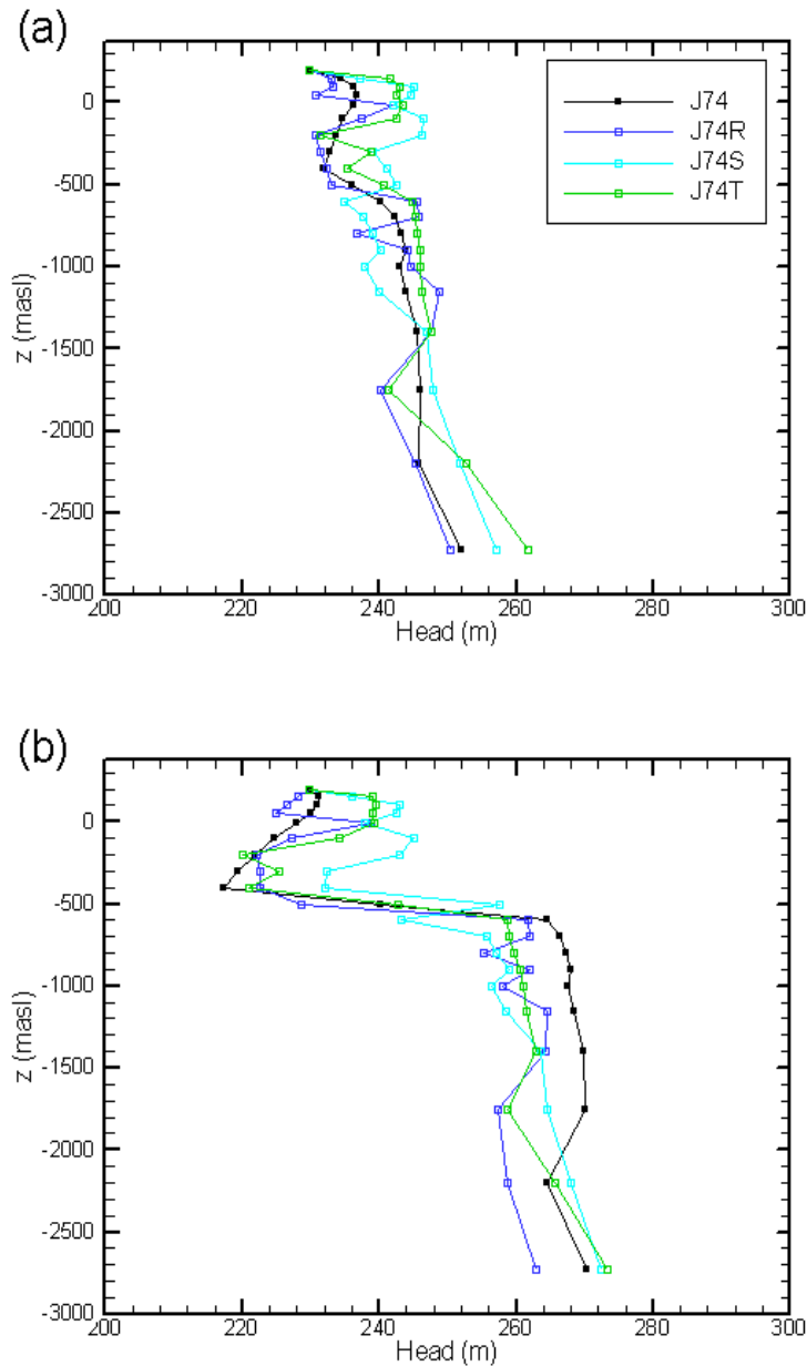
Figure 6. Head profiles at the location of Well MIU-2 for (a) the base case; and (b) the low-permeability Tsukiyoshi fault case. Cases J74R, J74S, and J74T represent different realizations of a random property distribution; Case J74 has uniform properties within each material type.
