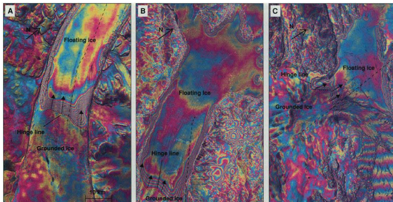
Fig. 2. Tidal displacements of the floating section of (A) Petermann Gletscher, (B) Nioghalvfjædsbræ Gletscher, and (C) Zachariae Isstrøm obtained from quadruple-difference ERS radar interferometry. Each fringe, or 360° variation in phase, represents a 28-mm displacement of the glacier tongue toward the radar line of sight (23° away from vertical) due to forcing by the ocean tide. The phase image is modulated by the radar brightness of the scene. The hinge line, or limit of tidal flexing, is shown as a dotted line. The amplitude of the tidal displacements raises quickly from the hinge line (high
