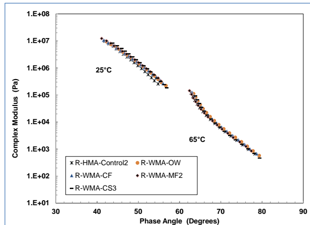
Figure 4.22: Phase 2, Mix Design #2: Black diagram for binders after 18 months.
