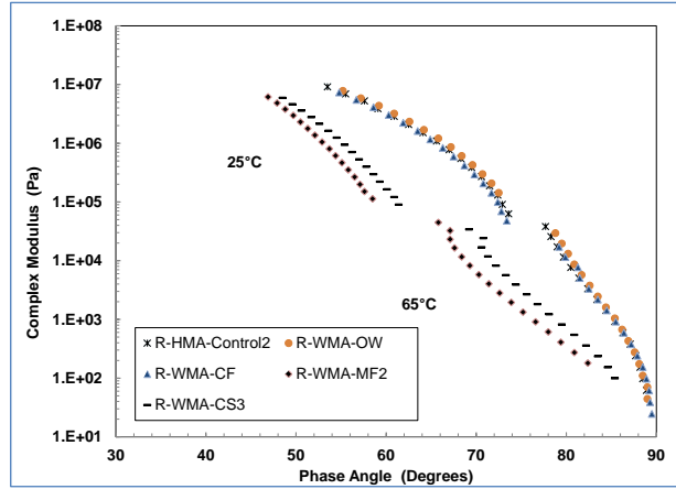
Figure 4.20: Phase 2, Mix Design #2: Black diagram for binders at zero aging (loose mix).
