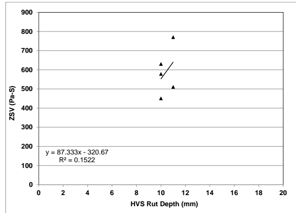
Figure 4.55: Phase 2, Mix Design #2: ZSV versus HVS rut depth.
