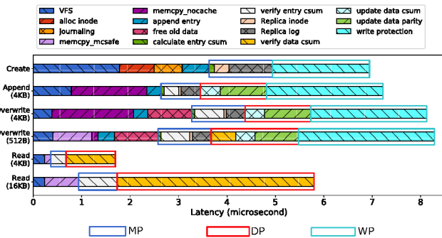
Figure 7: NOVA Latencies for NVDIMM-N For most operations, NOVA’s file data protection mechanisms have a larger impact on operation latencies that metadata protection, especially since the cost of verifying checksums scales with read and write size. For reads, in particular, verifying checksums increases latency by 70%.
