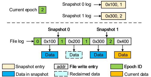
Figure 1: Taking snapshot in NOVA NOVA takes a snapshot by incrementing the epoch ID to start a new epoch. When a data block or log entry becomes dead in the current epoch, NOVA records its death in the snapshot log for most recent snapshot it survives in.
