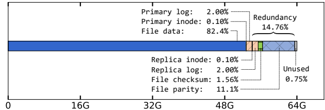
Figure 10: NVMM storage utilization. NOVA file system utilization by a large file server workload.
