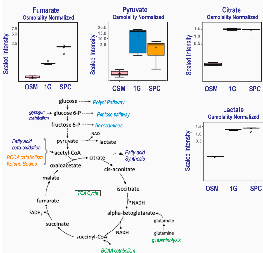
Figure 4. Comparison of metabolite utilization by 0G and 1G OLPs showed that in space, OLPs secreted significantly more fumarate than their 1G counterparts. OLPs from both groups secreted high levels of citrate and lactate, although with a slight but significantly higher level in 0G OLPs. ( n = 5 ). For box plots, whiskers reflect 5th and 95th percentiles (with the box displaying 25th to 75th quartiles); bisecting line represents the population median, while the plus sign (+) represents population mean; for details, see [21].
