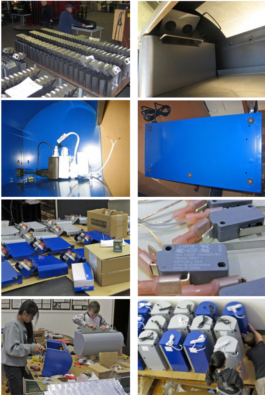
Figure 3.9: Images showing the fabrication, components and assembly of the footwarmer.
