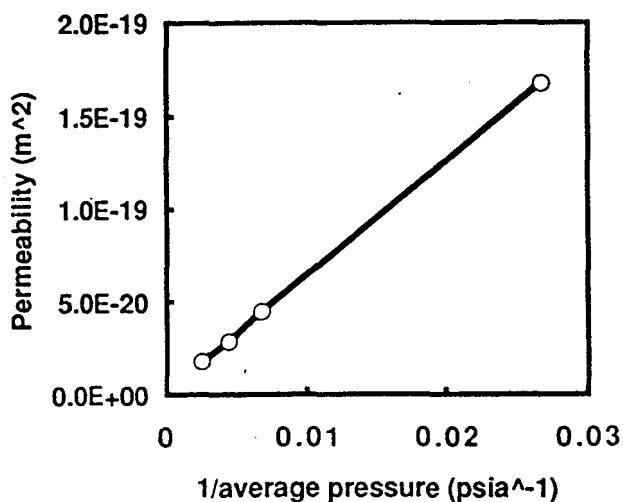
Figure 4. Klinkenberg plot of measured permeabilities for plug 26-2.
