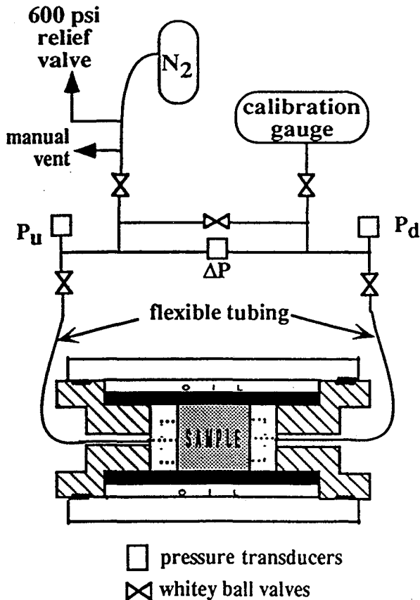
Figure 1. Gas-pressure-pulse-decay apparatus.
