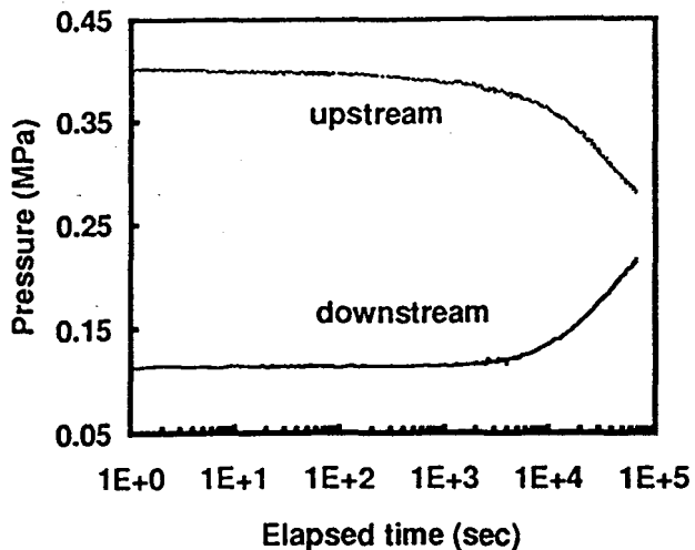
Figure 2. Pulse decay data for unfractured plug 54-1.
