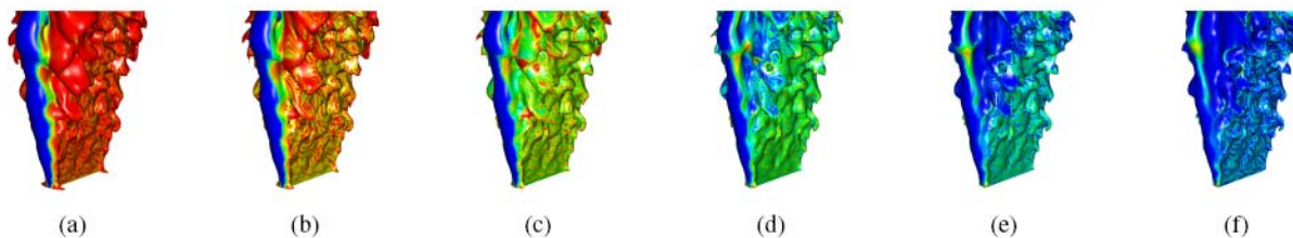
Figure 2. These images depict increase ((a) through (f)) isosurface values of temperature (isotherms) colored by values of the correlation field derived from water and ethylene. As temperature values increase, the predominant correlation between water and ethylene along the isotherms shifts away from strongly positive (red in (a)) to strongly negative (blue in (f)). This shift suggests that temperature is itself negatively correlated with the water-ethylene correlation. (Sample methane flame simulation data courtesy J. Bell and M. Day, Center for Computational Sciences and Engineering, LBNL)
