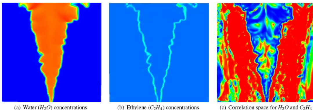
Figure 1. Water ( H_2O ) and ethylene ( C_2H_4 ) concentrations from the methane combustion dataset are shown in (a) and (b), respectively (Sample data courtesy J. Bell and M. Day, Center for Computational Sciences and Engineering, LBNL). The derived correlation field for these two compounds is shown in (c). The switch from strong positive correlation to strong negative correlation in the reaction region corresponds to the area in which C_2H_4 is both produced and consumed, and H_2O is produced, in the process of combustion. The strong correlation (both positive and negative) in the center of the flame, as well as the atmospheric region, demonstrates the correlation field’s ability to show fine-scale interactions.
