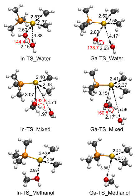
Figure 3. Ensemble averaged geometries for the transition state of both In and Ga nanocages. The simulation averaged geometric parameters (in units of Å, deg) are shown for Indium (left) and Gallium (right) capsules in pure water (top), mixture of 85% methanol and 15% water by volume (middle), and pure methanol solvent (bottom). Color key: carbon = grey, phosphorous = orange, gold = yellow, hydrogen = white, oxygen = red.
