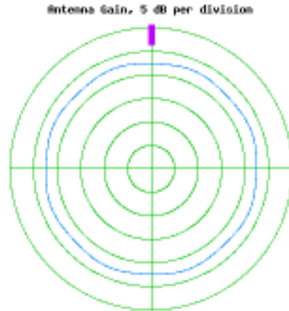
Figure 2.1: The beam pattern for an omnidirectional antenna. The line shows the relative beam strength at various angles to the Phocus Array. The distance the line is at any given point from the center of the graph indicates the magnitude of the beam at that angle. From Fidelity Comtech [3].
