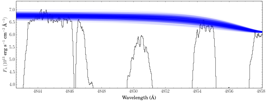
Figure 3.7. The 523 continua considered for estimation of the effect of continuum choice of D/H error in the vicinity of Ly \alpha . The 2\sigma continua uncertainty is 3% at \lambda = 4847.25 \text{ \AA} , beyond which the goodness of fit suffered significantly. In determining these continua, the fitting parameters for H I were locked since its fit is already well constrained by many observed Lyman-series transitions (see 3.4.1).
