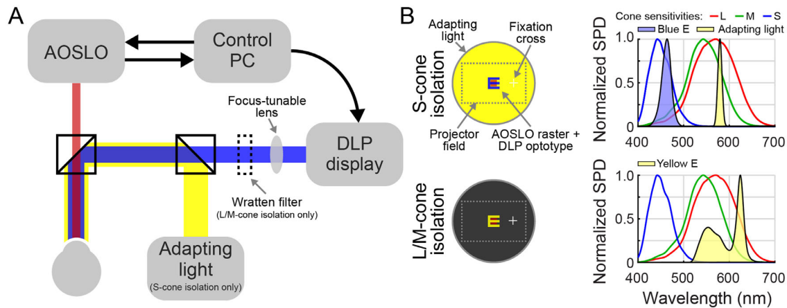
FIGURE 1. System schematic. (A) The psychophysical optotype E was delivered from the high-resolution Digital Light Processing (DLP) projector display through a different light path coaligned with the AOSLO beam. The focus of the letter E was adjusted with a focus-tunable lens subjectively. In the S-cone isolation condition, a background adapting light was created from an external light source coaligned with the projector path and AOSLO beam. The yellow adapting light was bright enough to desensitize the L/M-cones during S-cone acuity measurement. In the L/M-cone-isolating condition, a yellow letter E was created by filtering a white light through a long-pass Wratten 16 filter whose spectrum is outside of the sensitive region of the S-cones. (B) Cone isolation was achieved utilizing differences in spectral sensitivities. 85 In the S-cone-isolation condition, the subject viewed a blue letter E against a bright yellow background. In the L/M-cone-isolation condition, the subject viewed a yellow letter E against a black background. The red AOSLO IR raster was present and centered with the letter in both conditions.
