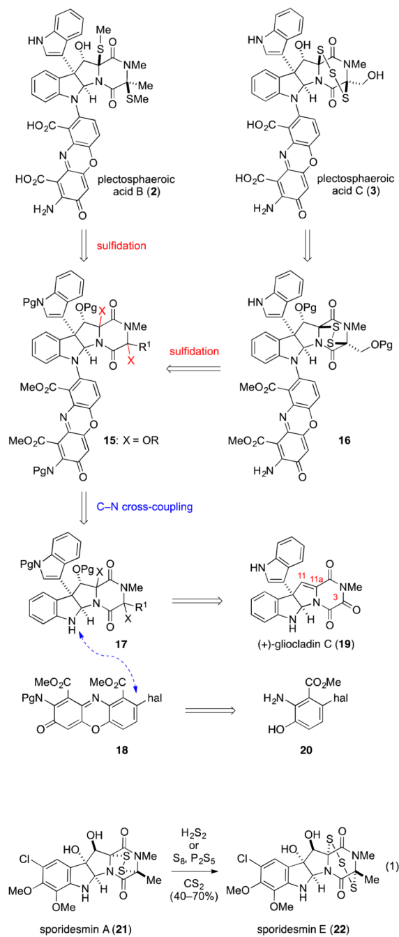
Scheme 1. Retrosynthetic Analysis of Plectosphaeroic Acids A–C
