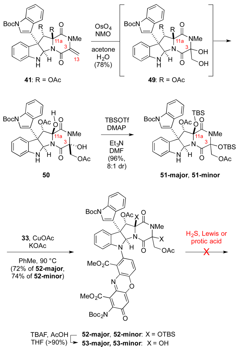
Scheme 9. Elaboration of Exo-methylene 41 to Intermediates 51 and 52
