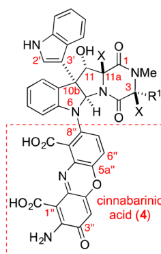
plectosphaeroic acid A: X = SMe, R 1 = CH 2 OH (1) B: X = SMe, R 1 = Me (2) C: X, X = -S 3 - , R 1 = CH 2 OH (3)
