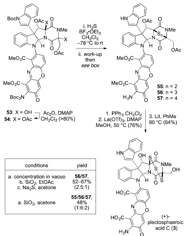
Scheme 10. Completion of the Total Synthesis of Plectosphaeric Acid C
