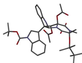
X-ray model of 40a
