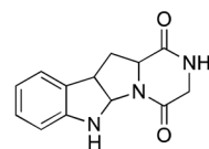
2,3,6,10b,11,11a-hexahydro-4 H -pyrazino-[1',2':1,5]-pyrrolo[2,3- b ]indole-1,4(5 aH )-dione (5)
