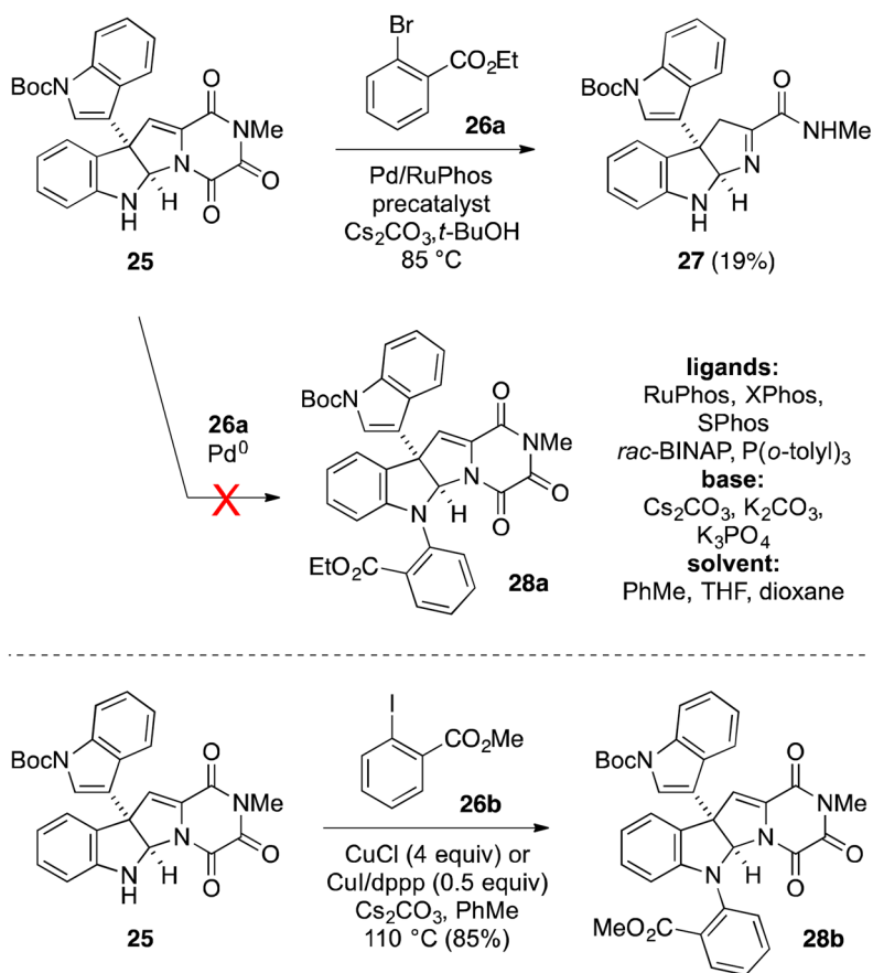
Scheme 2. Investigating Palladium(0)- and Copper(I)-Promoted C–N Cross-Coupling Reactions
