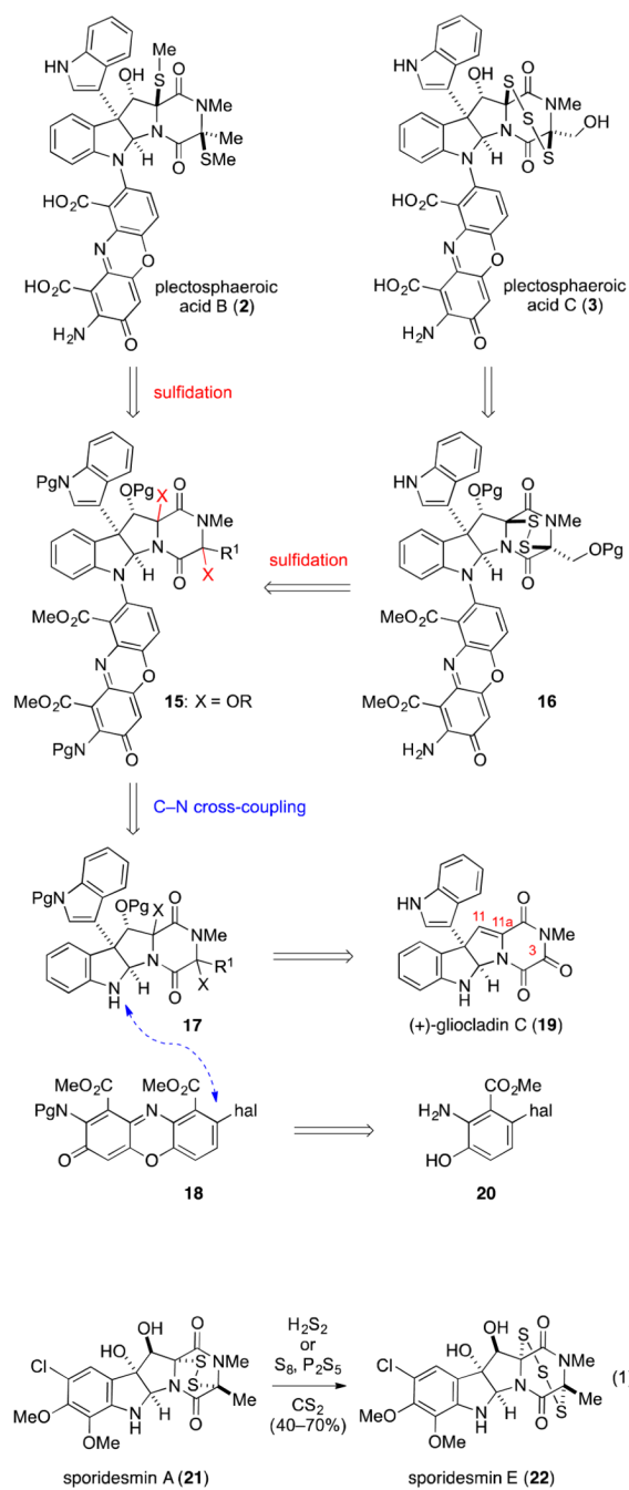
Scheme 1. Retrosynthetic Analysis of Plectosphaeroic Acids A–C
