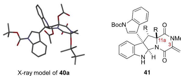
Scheme 5. Deprotection of the Indoline Nitrogen of 39a and 39b
