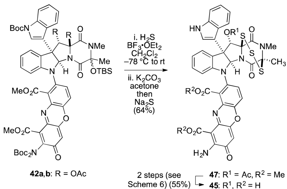
Scheme 8.
