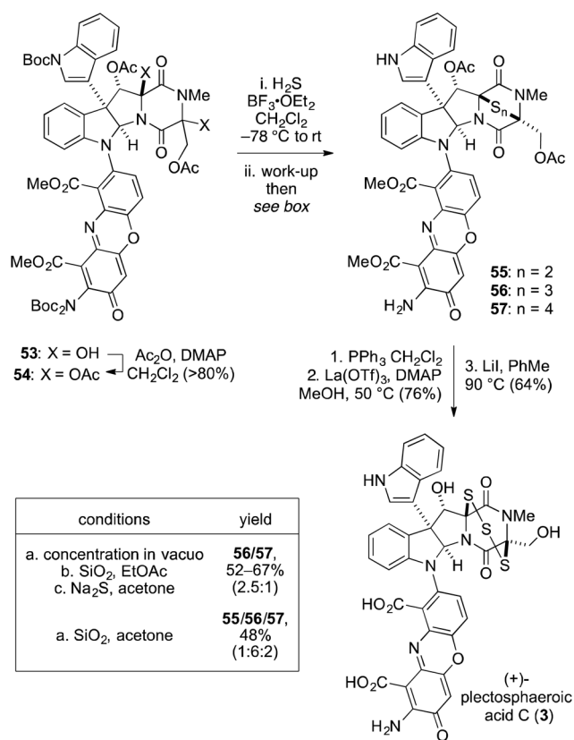
Scheme 10. Completion of the Total Synthesis of Plectosphaeroic Acid C
