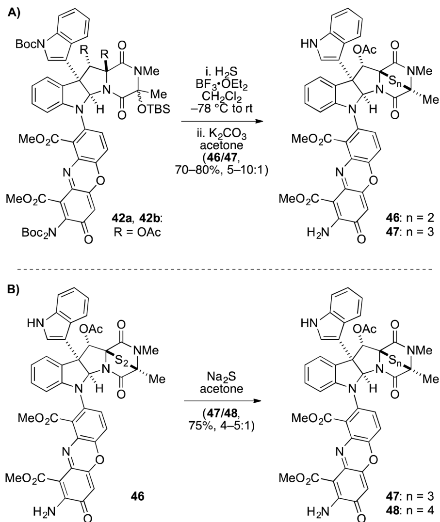
Scheme 7.
