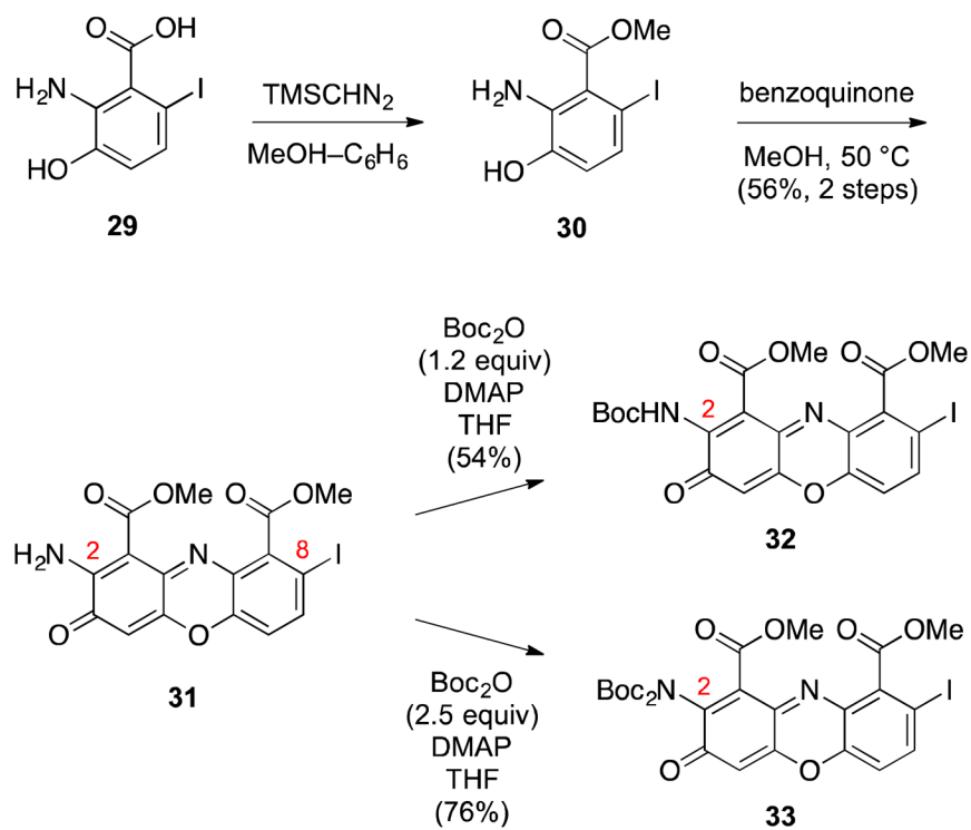
Scheme 3. Preparation of the 8-Iodophenoxazinone Coupling Partners
