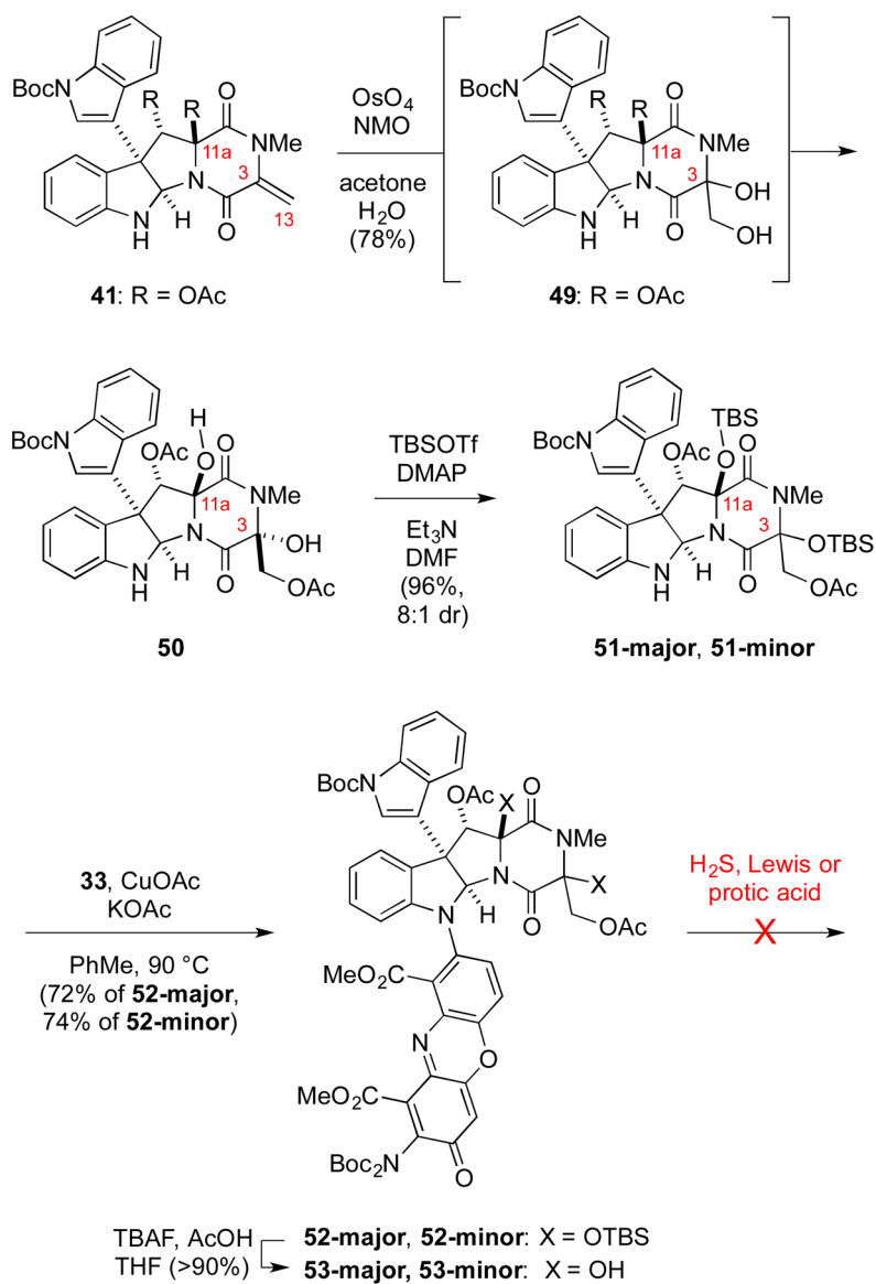
Scheme 9. Elaboration of Exo-methylene 41 to Intermediates 51 and 52
