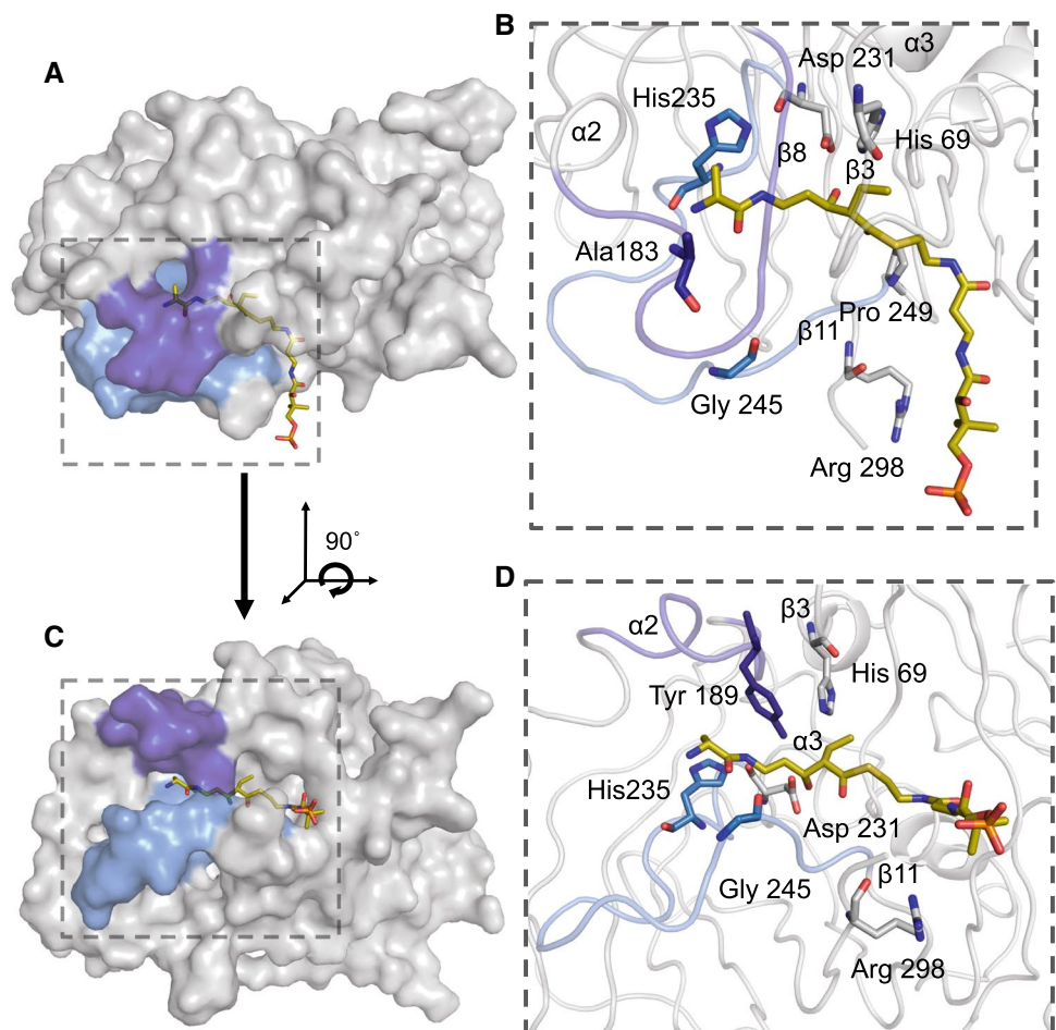
Fig. 4 In silico docking analysis of FluA DH M1 with the natural PPant-substrate intermediate 4 . Substrate 4 interacts with all three DH substrate-binding regions a . b A close inspection of the dipeptide moiety of 4 shows close interactions with residues located between \alpha 3 and \beta 11 (light blue) and \alpha 2 and \beta 8 (dark blue). c A 90° horizontal rotation of a and close-up of the substrate 4 and interacting residues (colour figure online)
