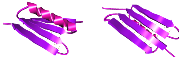
Figure 6: Two initial configurations for 1PGX.
