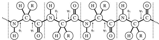
Figure 4: Rotational degrees of freedom along a residue chain. Adjacent residues are separated by dashed lines; side chains are denoted by R.
