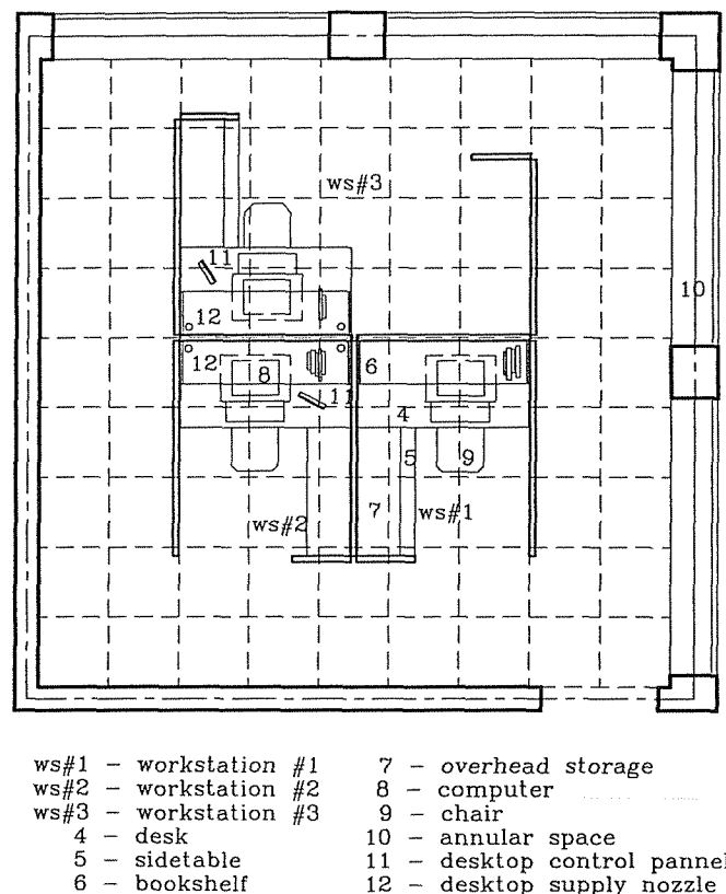
Figure 3 Controlled environment chamber plan.
