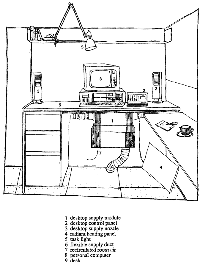
Figure 1 Desktop task conditioning system.
