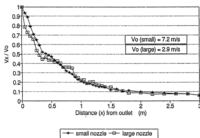
Figure 4 Centerline velocity profile: Isothermal conditions, supply volume = 55 cfm.
