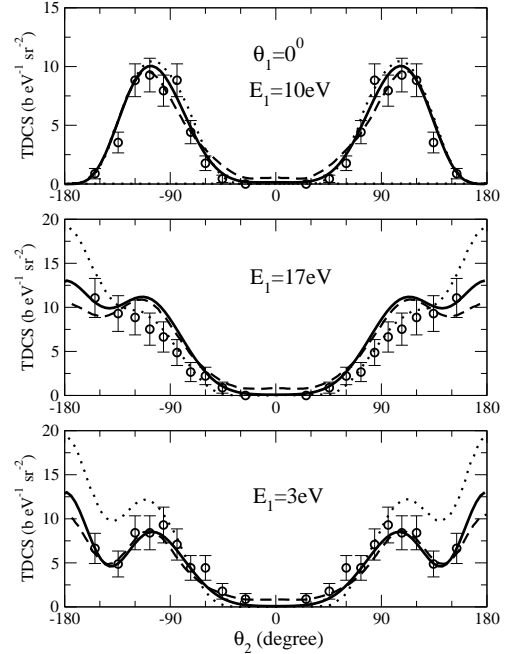
FIG. 5: TDCS for photon energy 20 eV above threshold, at various energy sharings for \theta_1 = 0^0 . Circles: experiment by Bräuning et al. [2]. Dashed curve: TD-CC calculations by Colgan et al. [22]. Dotted curve: HRM-SOW calculations by Selles et al. [20]. Thick solid curve: Present result.
