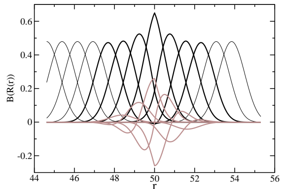
FIG. 1: 8th order B-splines on the complex exterior scaling contour with R_0 = 50 and \eta = 40^\circ . Heavy black lines are the real parts of the only complex splines. Grey lines are the imaginary parts.
