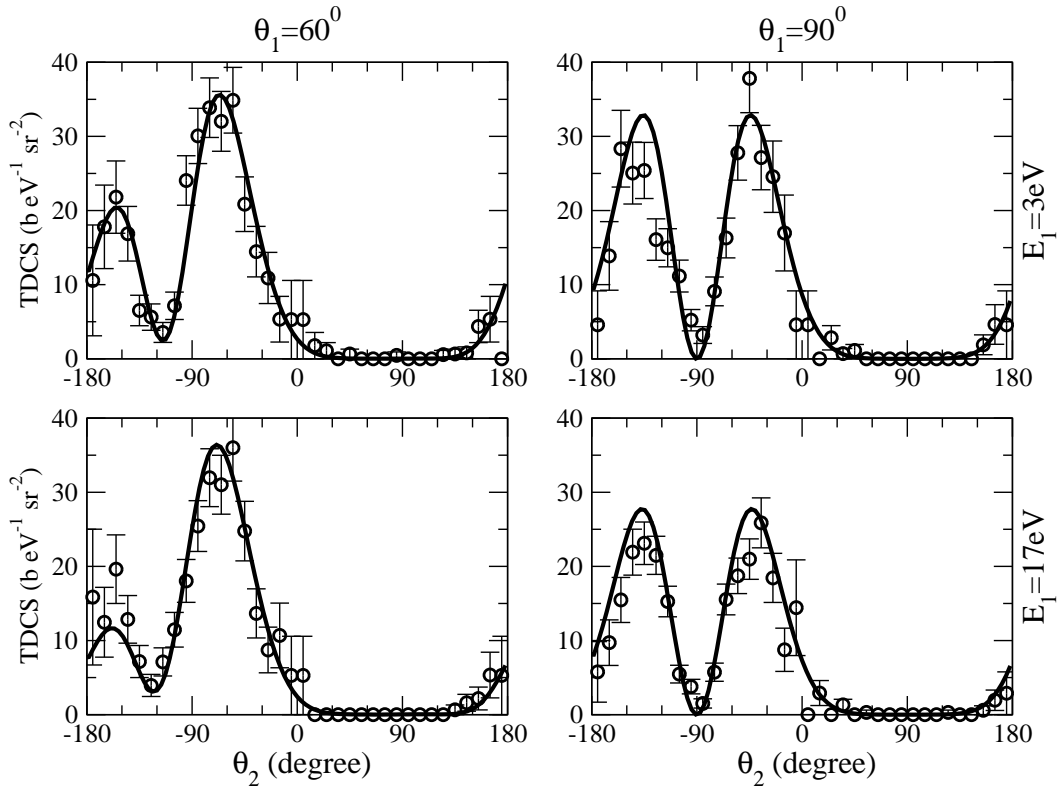
FIG. 7: TDCS for photon energy 20 eV above threshold, at energy sharings with E_1 = 3\text{eV} (upper panels) and 17 eV (lower panels) for \theta_1 = 60^\circ and \theta_1 = 90^\circ . Circles: experiment by Braüning et al. [2]. Thick solid curve: Present result.
