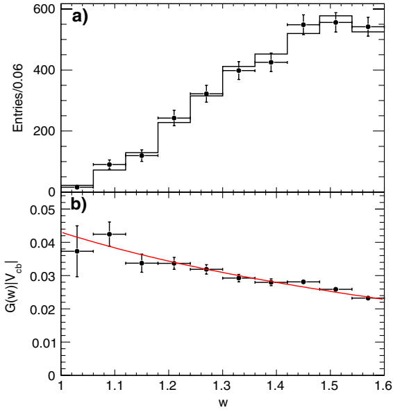
FIG. 2 (color online). (a) Signal yield w distribution obtained summing B^- \rightarrow D^0 \ell^- \bar{\nu}_\ell and \bar{B}^0 \rightarrow D^+ \ell^- \bar{\nu}_\ell events. The data ( \bullet ) are compared to the results of the overall fit (histogram). (b) \mathcal{G}(w)|V_{cb}| distribution corrected for the reconstruction efficiency, with the fit result superimposed.
