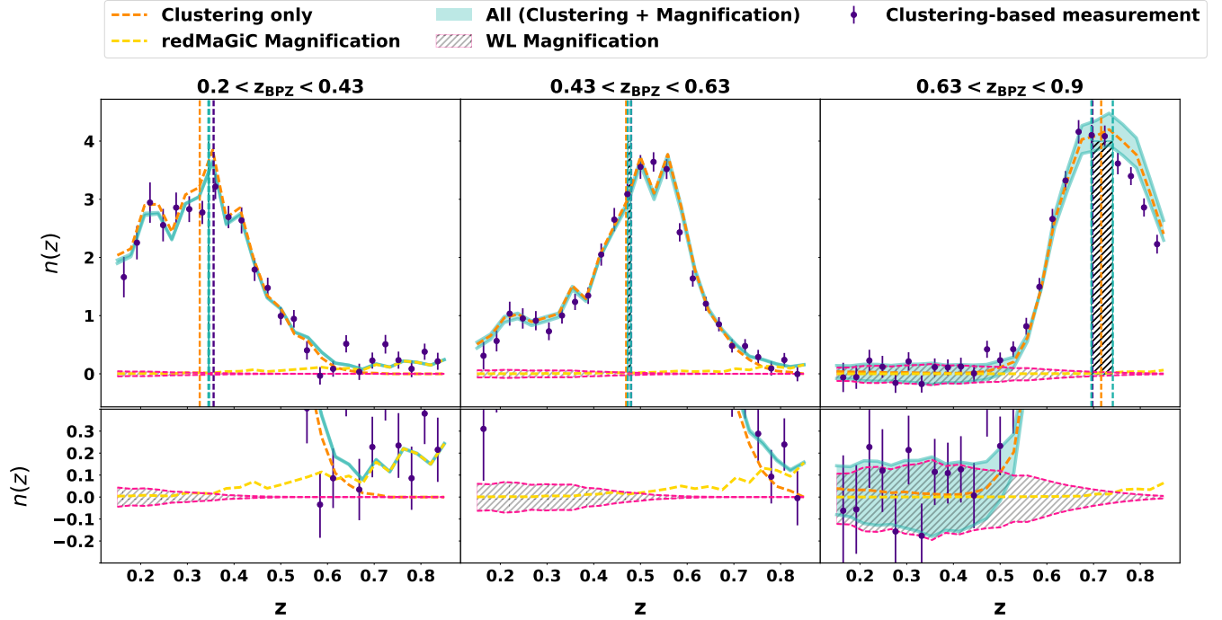
Figure 8. Upper panels: Effect of lensing magnification on clustering-based estimate. Shaded regions represent theoretical predictions for the various components of the signal (lensing magnification due to redMaGiC and the WL sample, as well as the clustering due to gravitational interaction only), while the points represent the actual measurement in simulations. Vertical lines show the mean of the redshift distributions computed over the full redshift interval. Lower panels: as the upper panels, but zoomed in on the lensing magnification signal.
