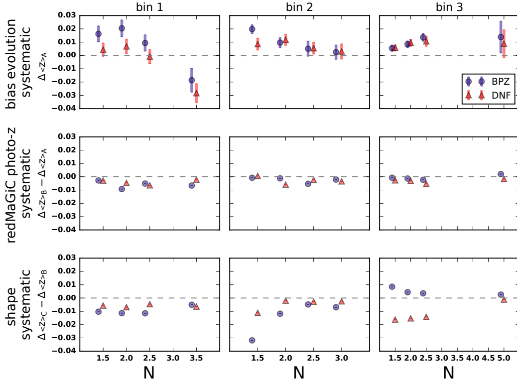
Figure 5. Mean matching procedure: inferred values of the three systematics as a function of matching interval, defined as \langle z \rangle_{WZ} \pm N\sigma_{WZ} . For each WL redshift bin, we show results for N=1.5, N=2 and N=2.5 ; in addition, we show results obtained including all the redshift interval covered by redMaGiC galaxies. This corresponds to N=3.5, N=3 and N=5 for the 1st, 2nd and 3rd source redshift bin respectively. For the 3rd bin a larger N is needed to include the low redshift tail down to z=0.15 .
